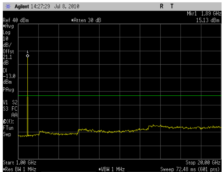
Plot 7.2 -10 (8PSK Ch661)
