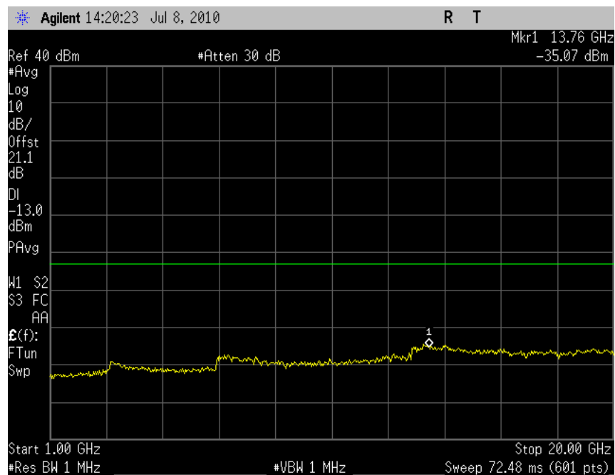
Plot 7.2 -16 (8PSK Ch190)
