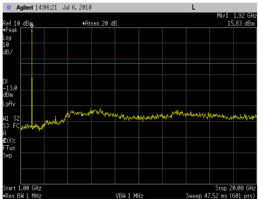
Plot 7.2 - 54 (EVDO, Rel 0, Ch. 1175)
