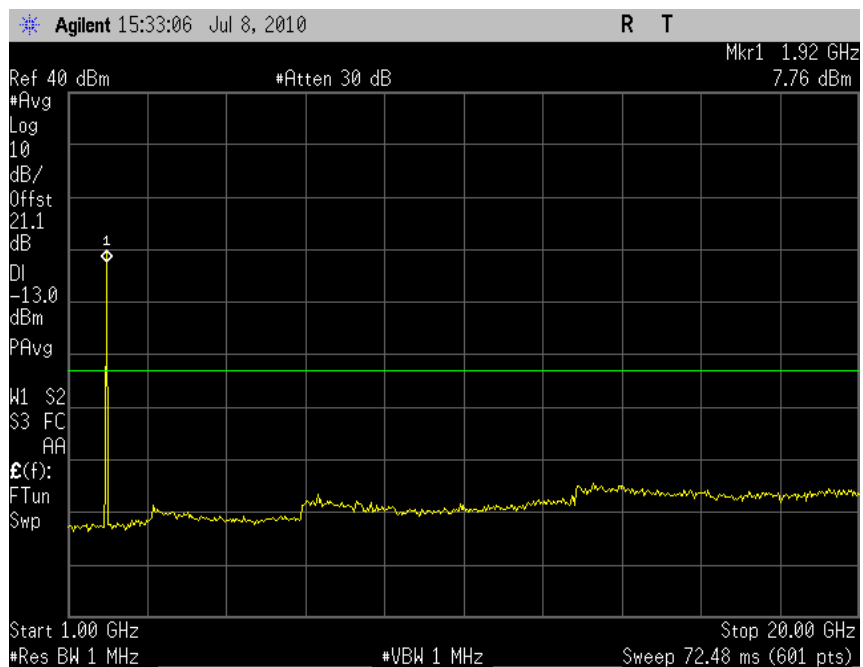
Plot 7.2 - 42 (Rel99, Ch9538)
