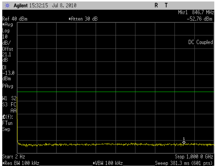
Plot 7.2 - 42 (Rel99, Ch9538)
