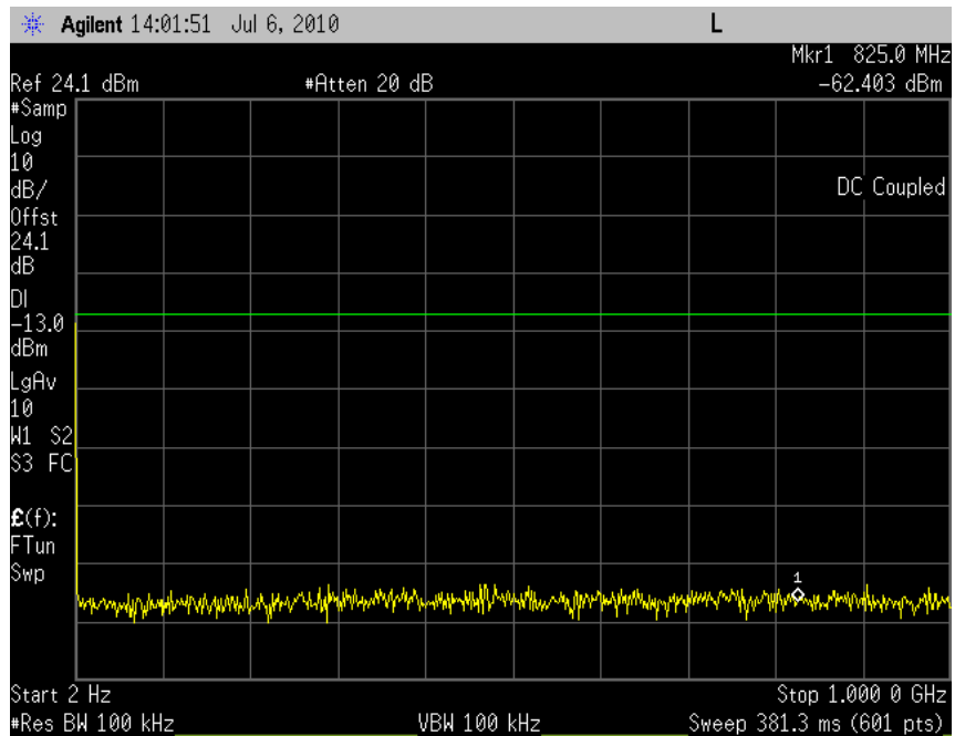
Plot 7.2 - 54 (EVDO, Rel 0, Ch. 1175)
