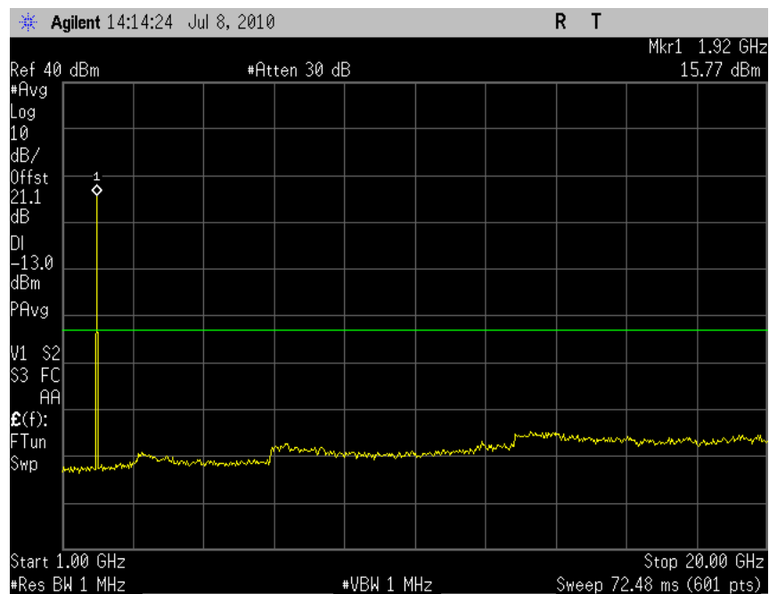
Plot 7.2 - 24 (8PSK Ch810)
