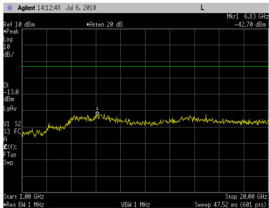
Plot 7.2 -46 (EVDO, Rel 0, Ch. 384)
