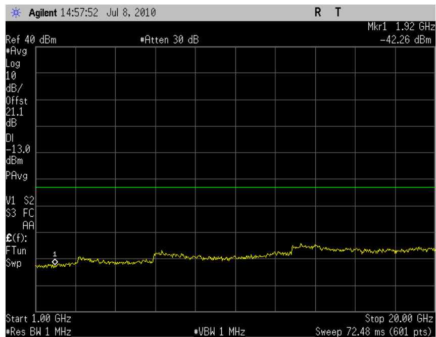
Plot 7.2 - 4 (8PSK Ch190)
