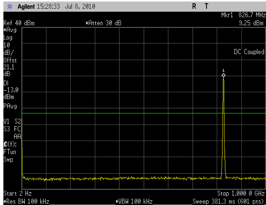
Plot 7.2 - 26 (Rel99, Ch4132)
