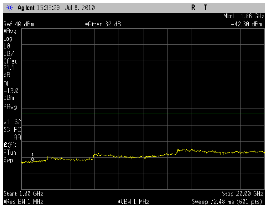
Plot 7.2 - 28 (Rel99, Ch4182)
