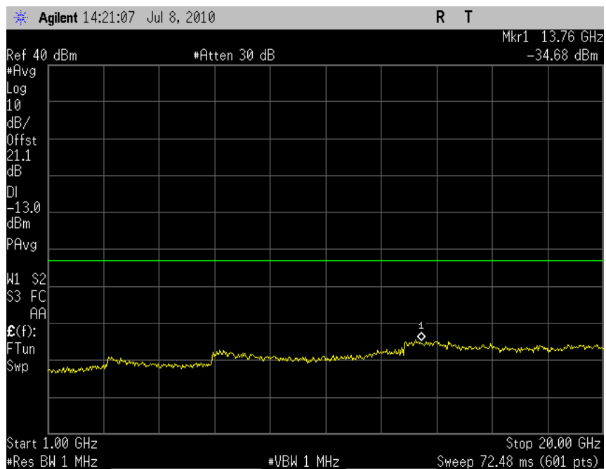
Plot 7.2 -14 (8PSK Ch128)
