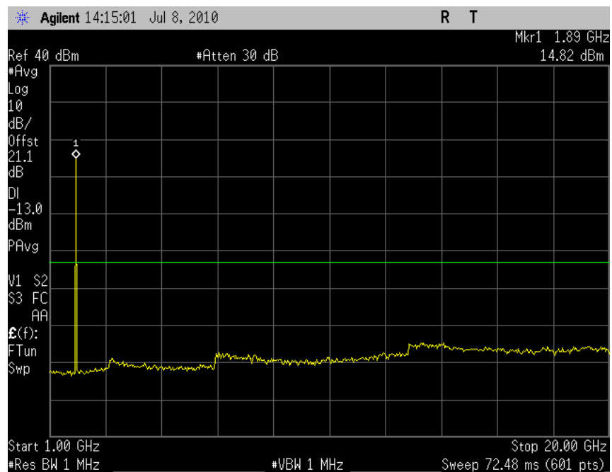
Plot 7.2 - 22 (8PSK Ch661)
