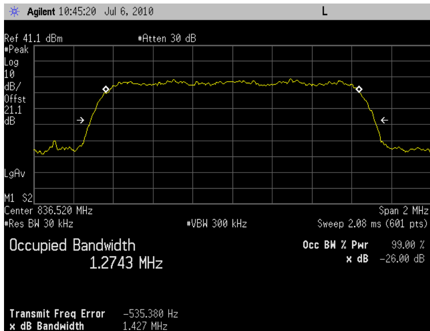
Plot 5.2-32 (Ch. 384, RC3 SO55)
