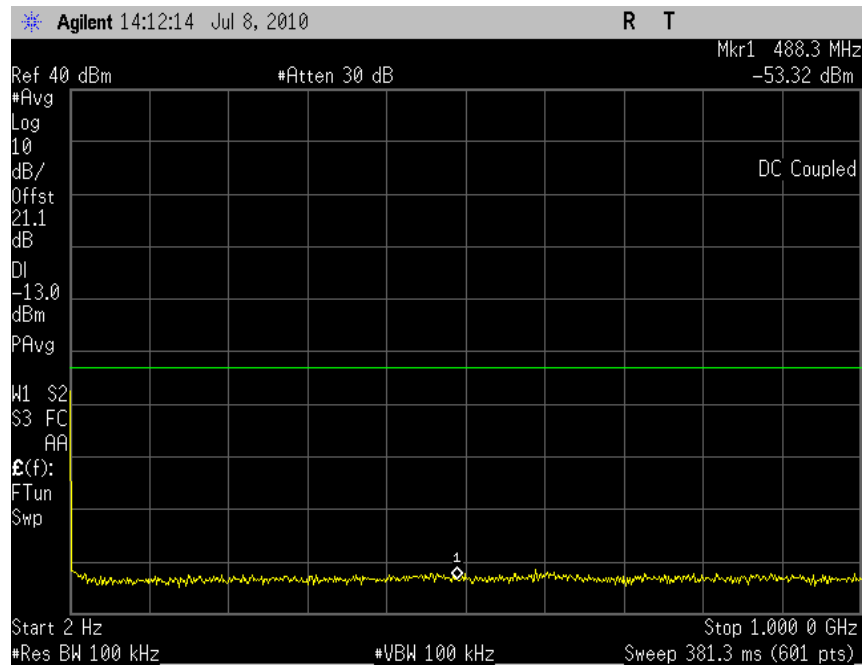
Plot 7.2 - 24 (8PSK Ch810)
