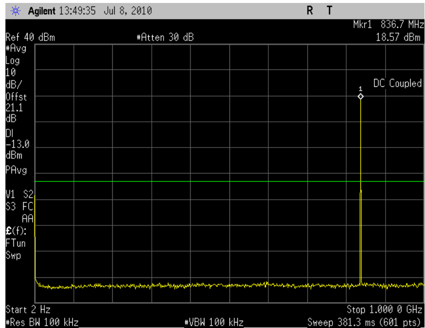
Plot 7.2 -16 (8PSK Ch190)
