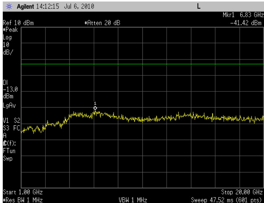
Plot 7.2 -44 (EVDO, Rel 0, Ch. 1013)
