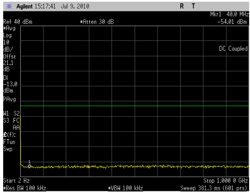
Plot 7.2 - 34 (Rel99, Ch1427)
