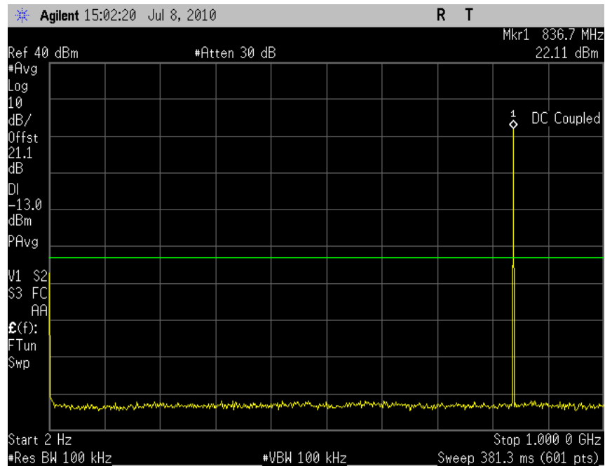
Plot 7.2 - 4 (8PSK Ch190)
