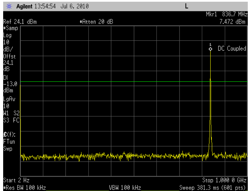
Plot 7.2 -46 (EVDO, Rel 0, Ch. 384)
