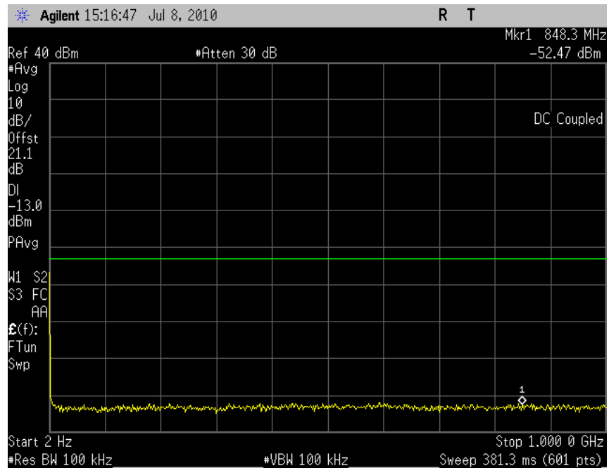
Plot 7.2 -10 (8PSK Ch661)
