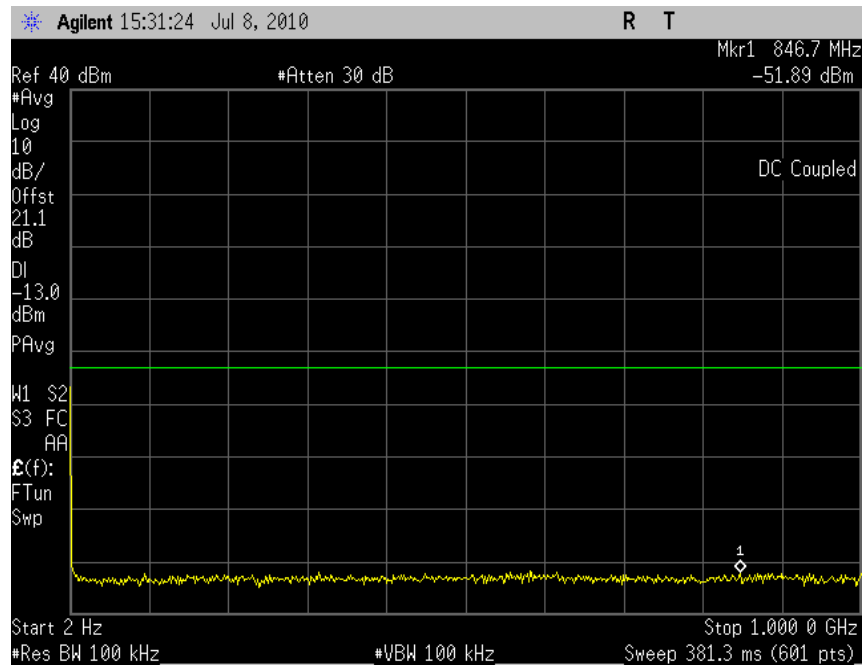
Plot 7.2 - 38 (Rel99, Ch9262)
