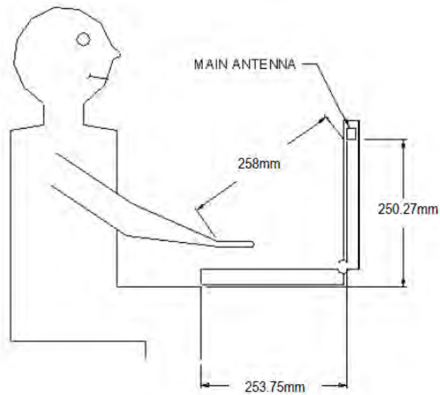
Fig.12 Antenna location of EUT (laptop mode)
