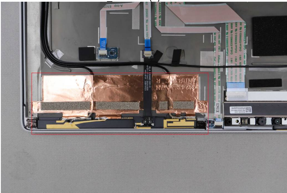
WWAN Antenna (1) for Vendor 2
