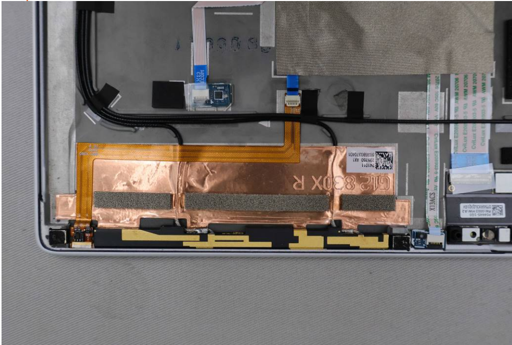
WWAN Antenna (1) for Vendor 1
