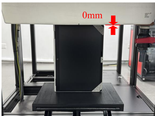
Photograph 7. Body, Left Edge, 0mm
