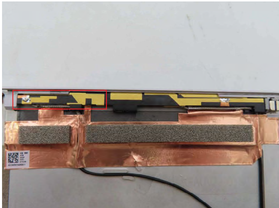
WLAN AUX Antenna for Vendor 2
