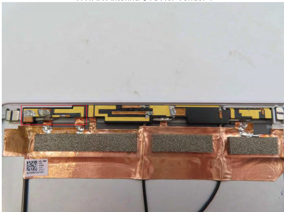
WWAN Antenna 6 RX for Vendor 1
