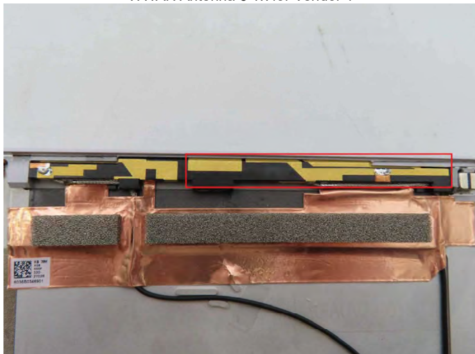
WWAN Antenna 5 Tx for Vendor 1
