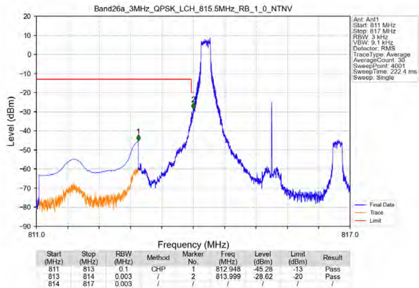
Band26a_3MHz_QPSK_LCH_815.5MHz_RB_1_0_NTNV
