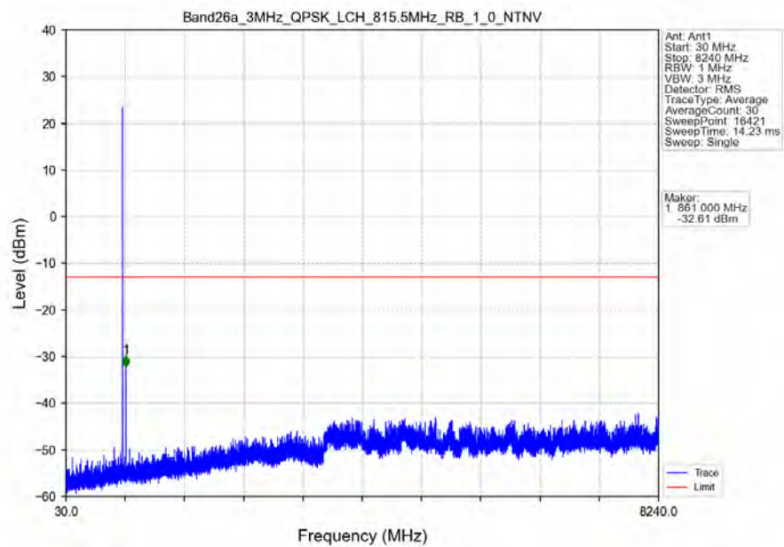
Band26a_3MHz_QPSK_LCH_815.5MHz_RB_1_0_NTNV
