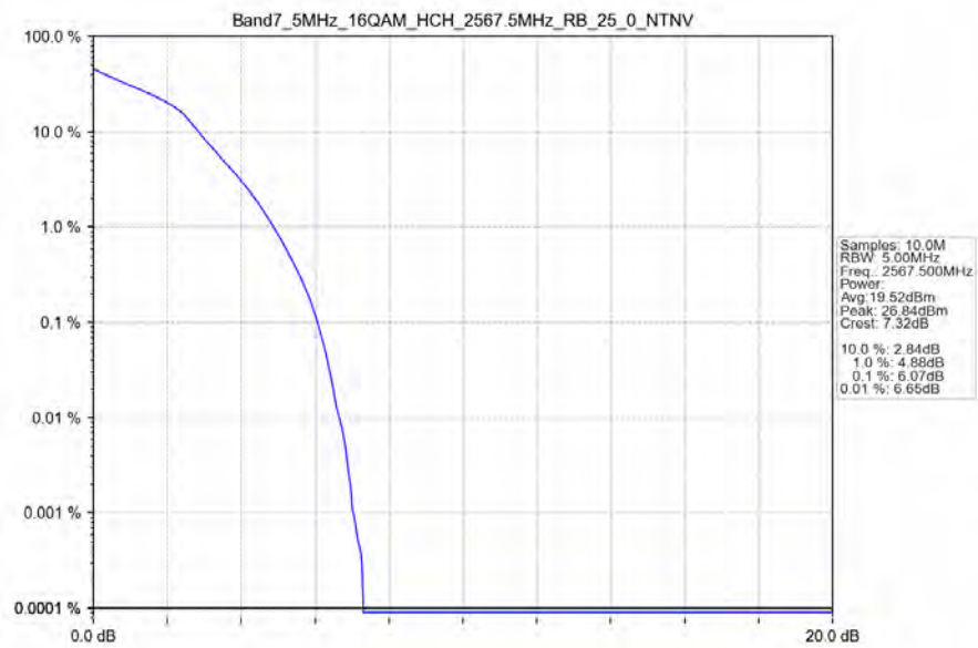
Band7_5MHz_16QAM_HCH_2567.5MHz_RB_25_0_NTNV
