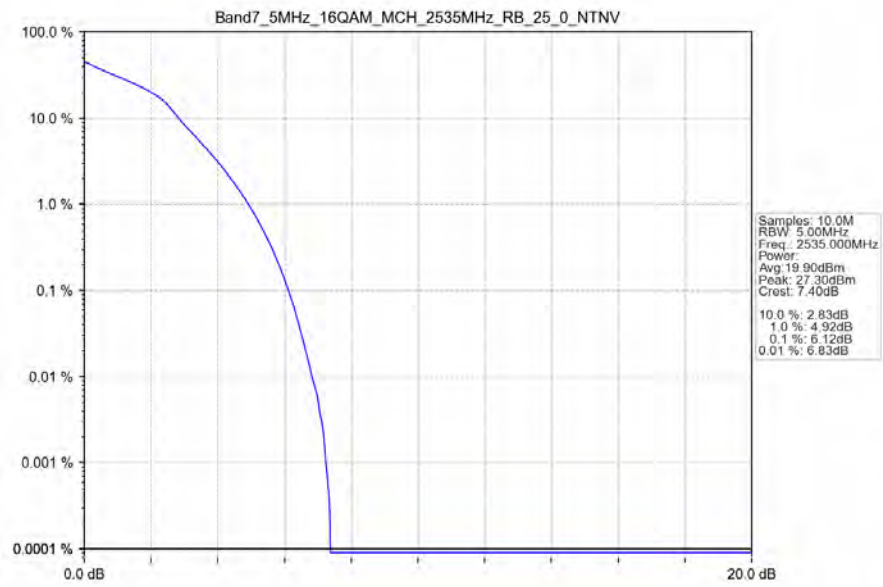
Band7_5MHz_16QAM_MCH_2535MHz_RB_25_0_NTNV
