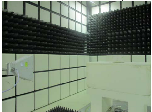
Part 22 24 27 Cat M1 Radiated NB Setup
