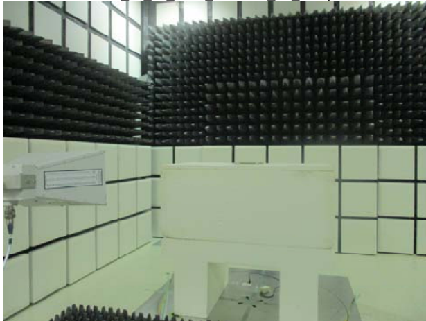
Part 22_24 GSM Radiated E2 Setup
