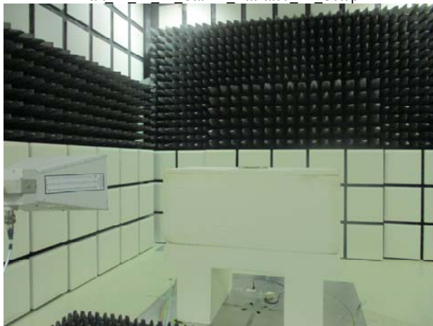
Part 22 24 27 Cat M1 Radiated E2 Setup
