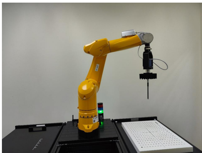
Fig.1 Photograph of the SAR measurement system
