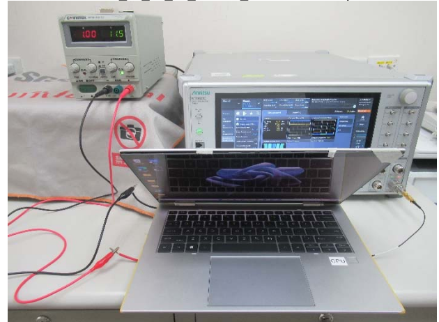
FCC 22 24 27 Cat-M1 Conducted Setup
