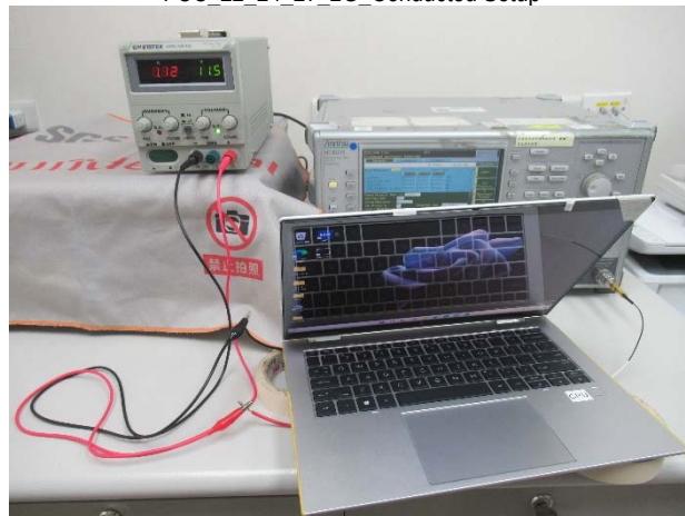
FCC 22 24 27 2G_Conducted Setup
