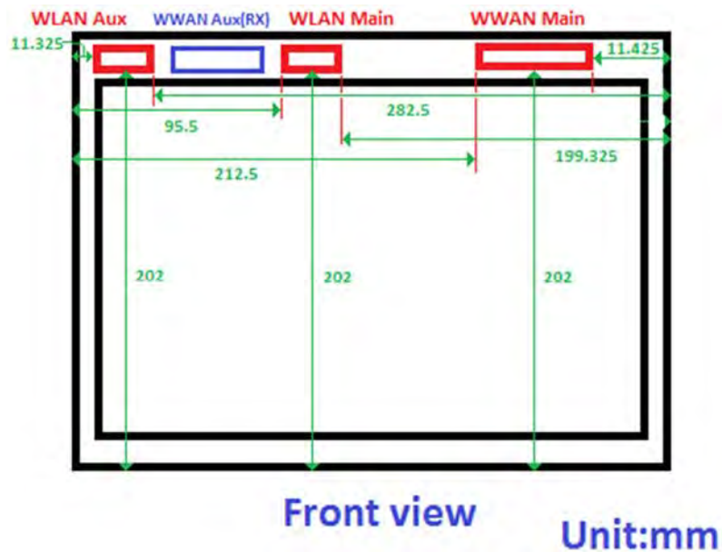
Fig.10 Antenna location of EUT (tablet mode)
