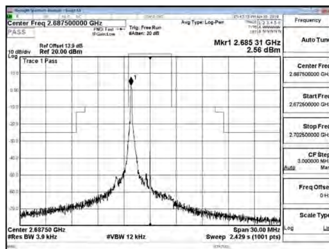
Band41_5MHz_16QAM_1_0_CH41565
