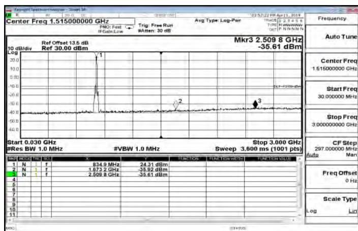
30MHz~3GHz_HSUPA_B5_MidCH4183-836.6
