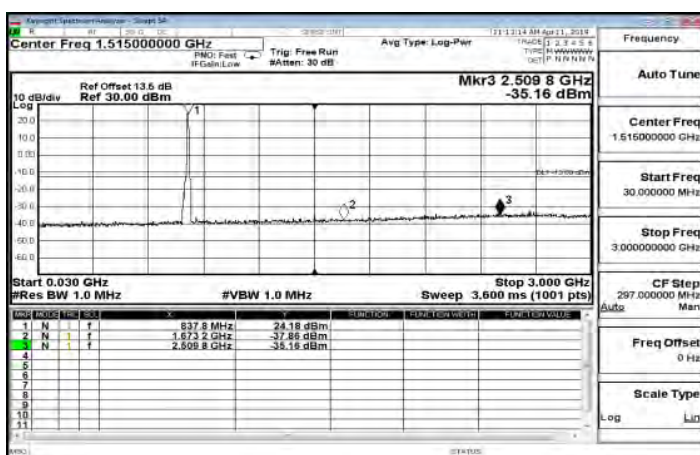
30MHz~3GHz_WCDMA_B5_MidCH4183-836.6
