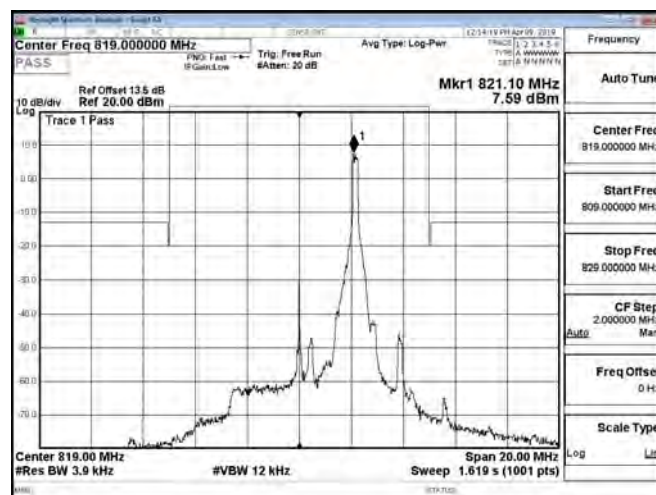
Band26_Part90s_5MHz_QPSK_1_24_CH26765
