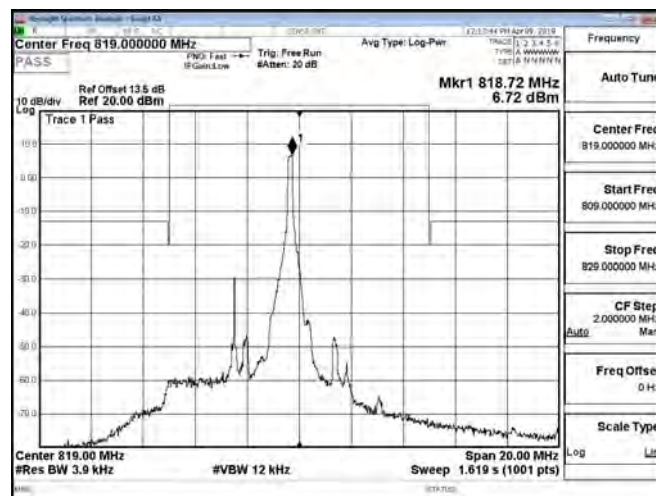
Band26_Part90s_5MHz_QPSK_1_24_CH26740
