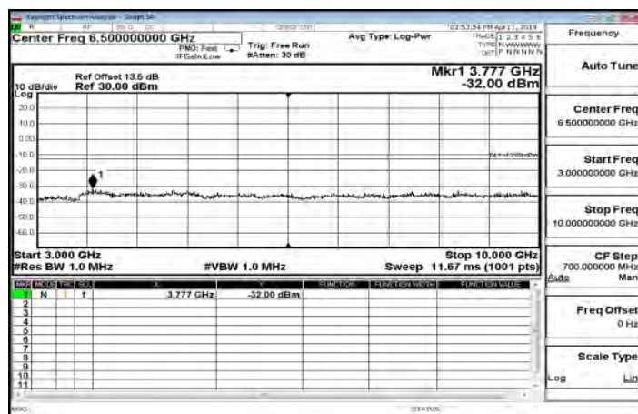
3GHz~10GHz_HSUPA_B5_HighCH4233-846.6
