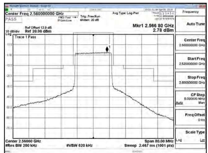
Band7_20MHz_16QAM_100_0_CH21350
