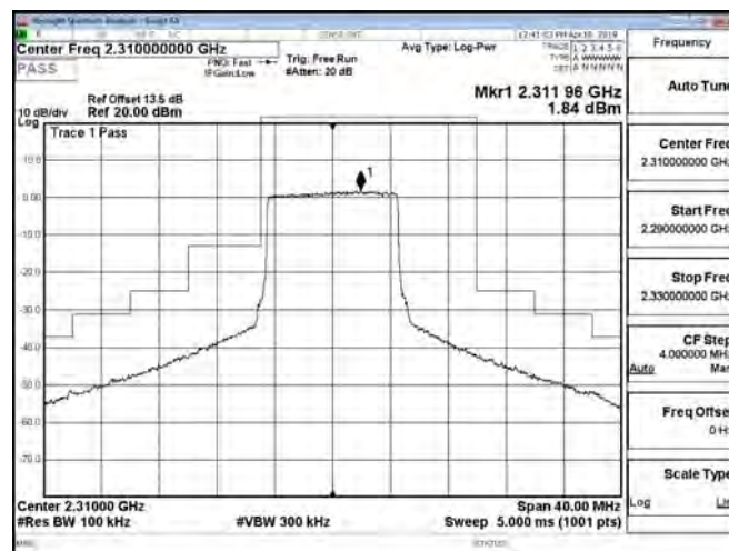
Band30_10MHz_16QAM_50_0_CH27710
