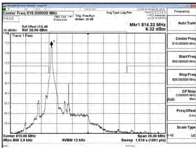
Band26_Part90s_5MHz_QPSK_1_0_CH26740
