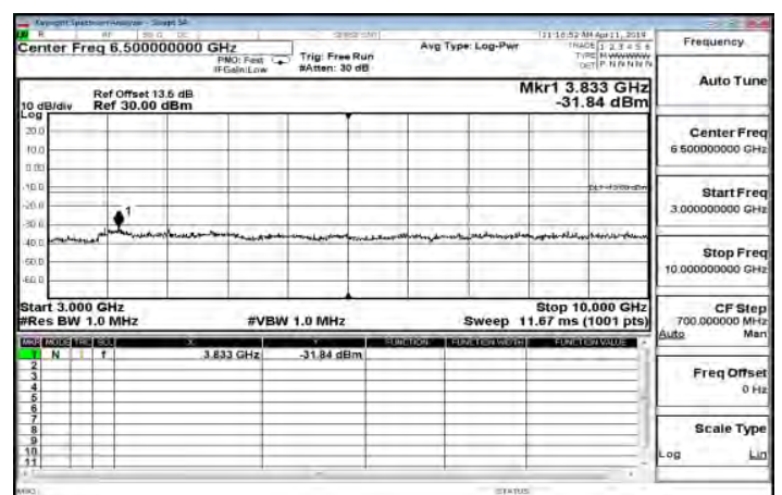
3GHz~10GHz_WCDMA_B5_HighCH4233-846.6
