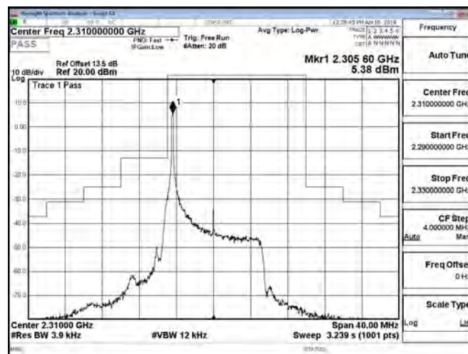
Band30_10MHz_16QAM_1_49_CH27710
