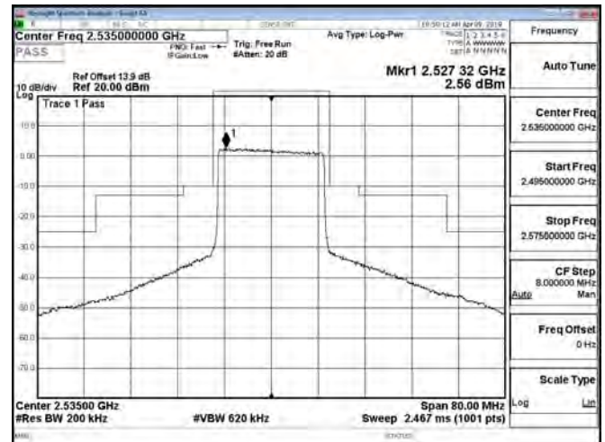
Band7_20MHz_16QAM_100_0_CH21350
