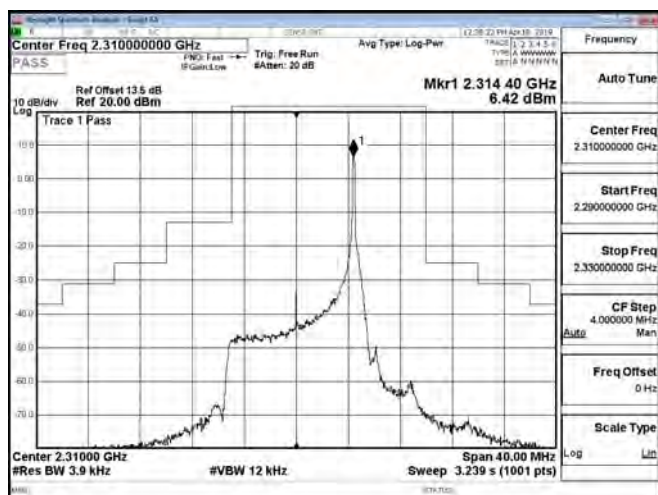
Band30_10MHz_QPSK_50_0_CH27710
