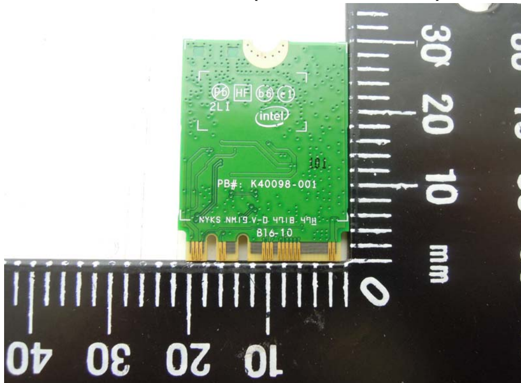
WLAN / BT Module-3 (Model No.: AX200NGW)
