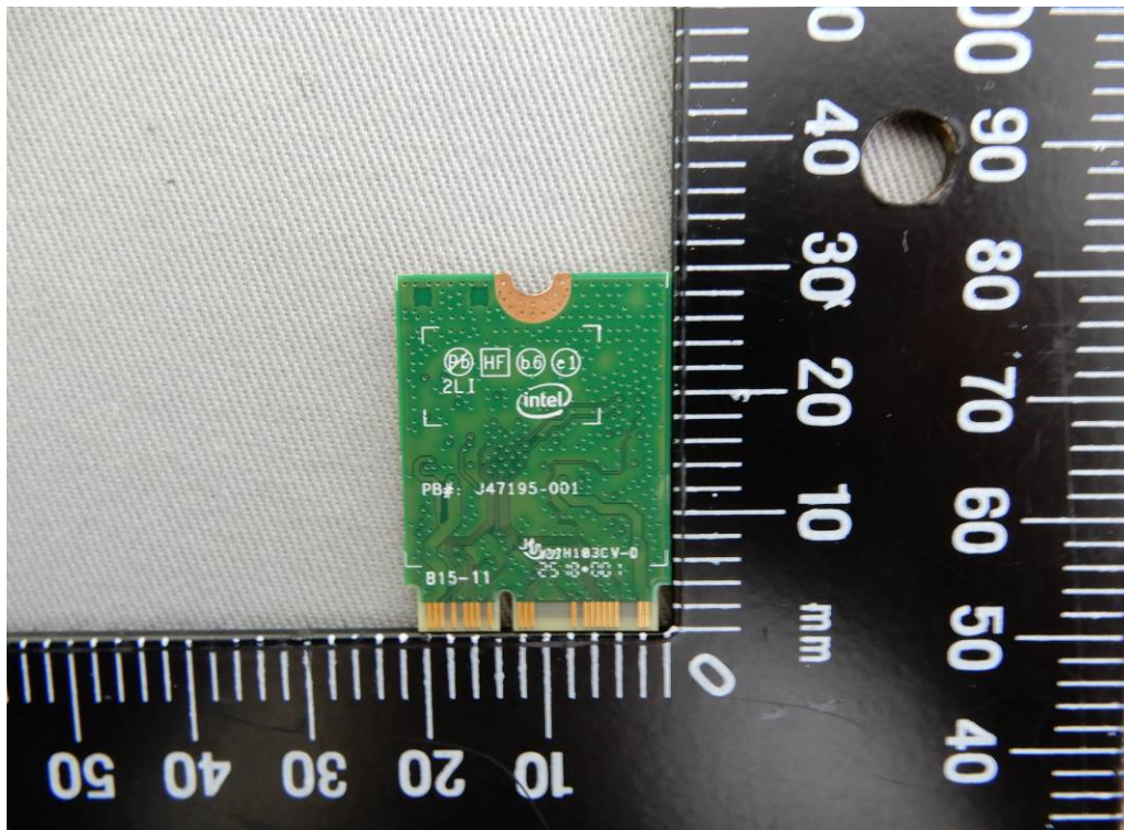
WLAN / BT Module-2 (Model No.: 9560NGW)
