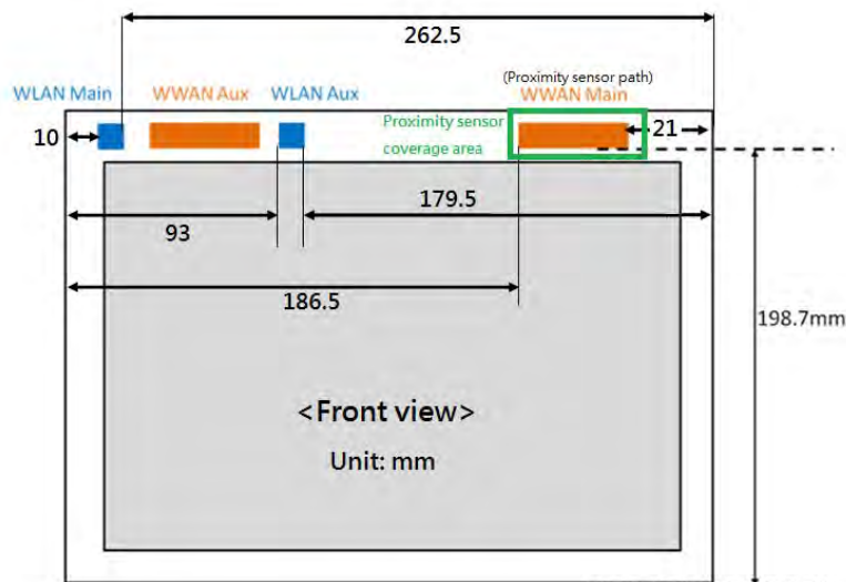
Fig.11 Antenna position of EUT (Front view)
