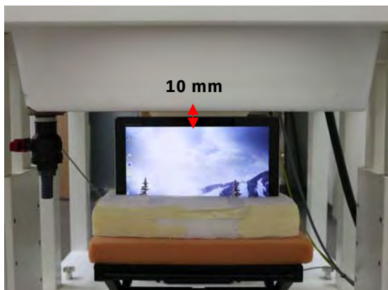
Fig.7 EUT Top side (10mm) to flat phantom
