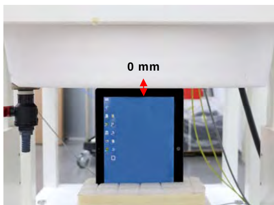
Fig.4 EUT Right side to flat phantom
