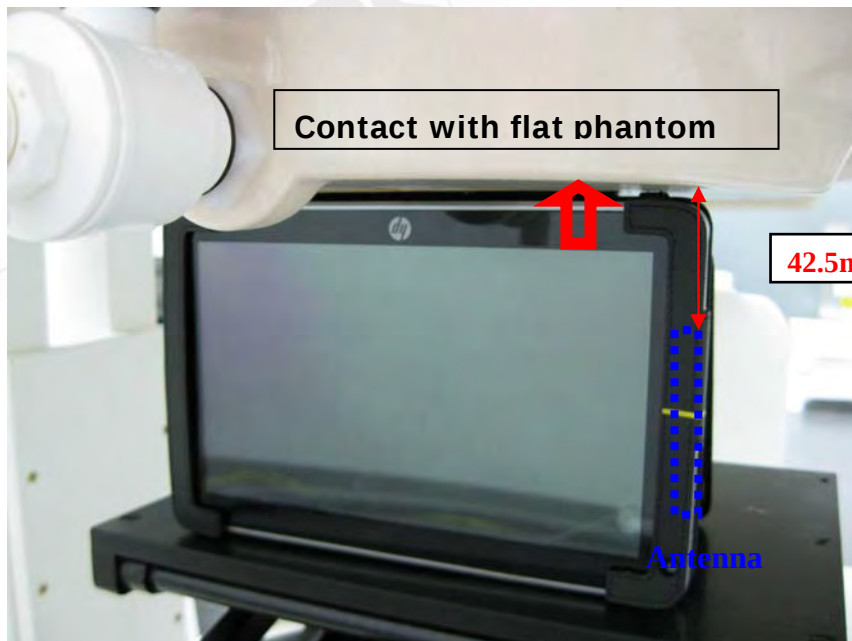
Fig.7 Primary Landscape mode
