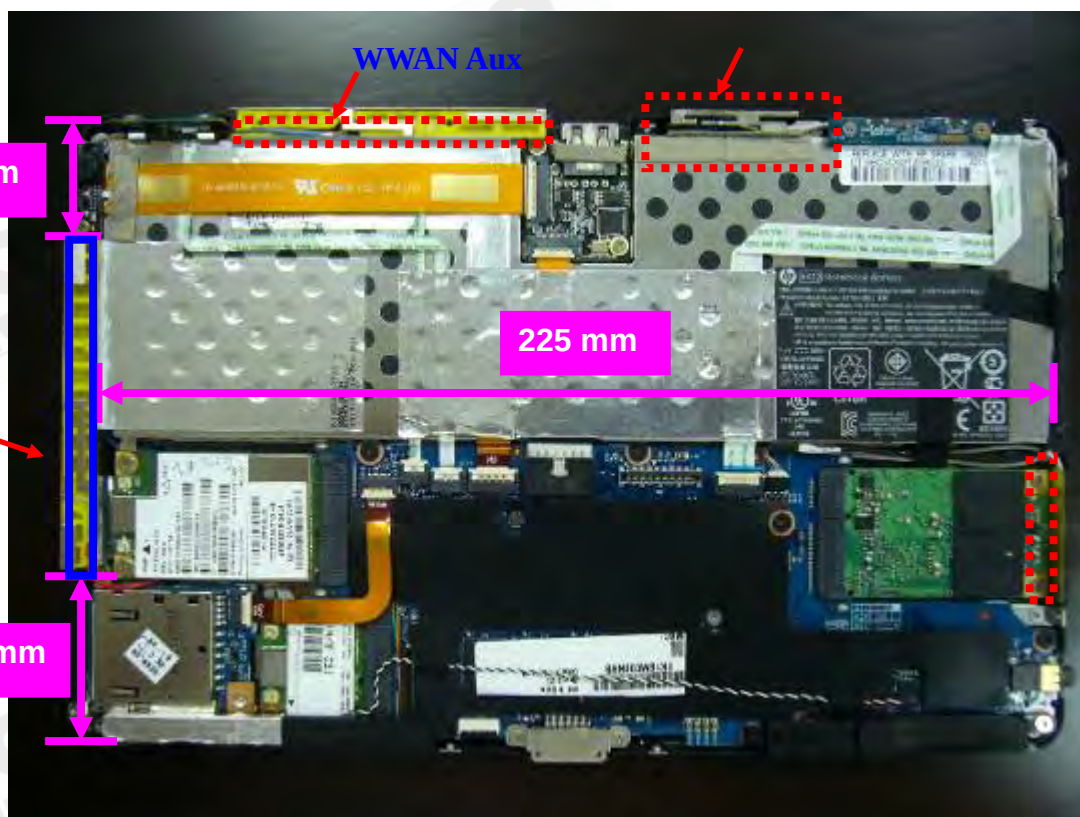
Fig.13 Antenna position of EUT
