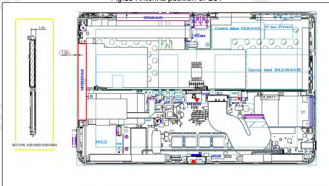
Fig.14 Antenna position of EUT
