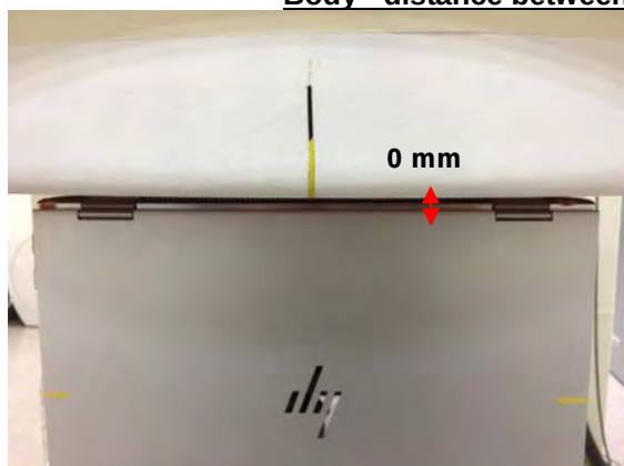
Fig.6 EUT Laptop mode to flat phantom
