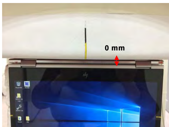
Fig.7 EUT stand mode to flat phantom
