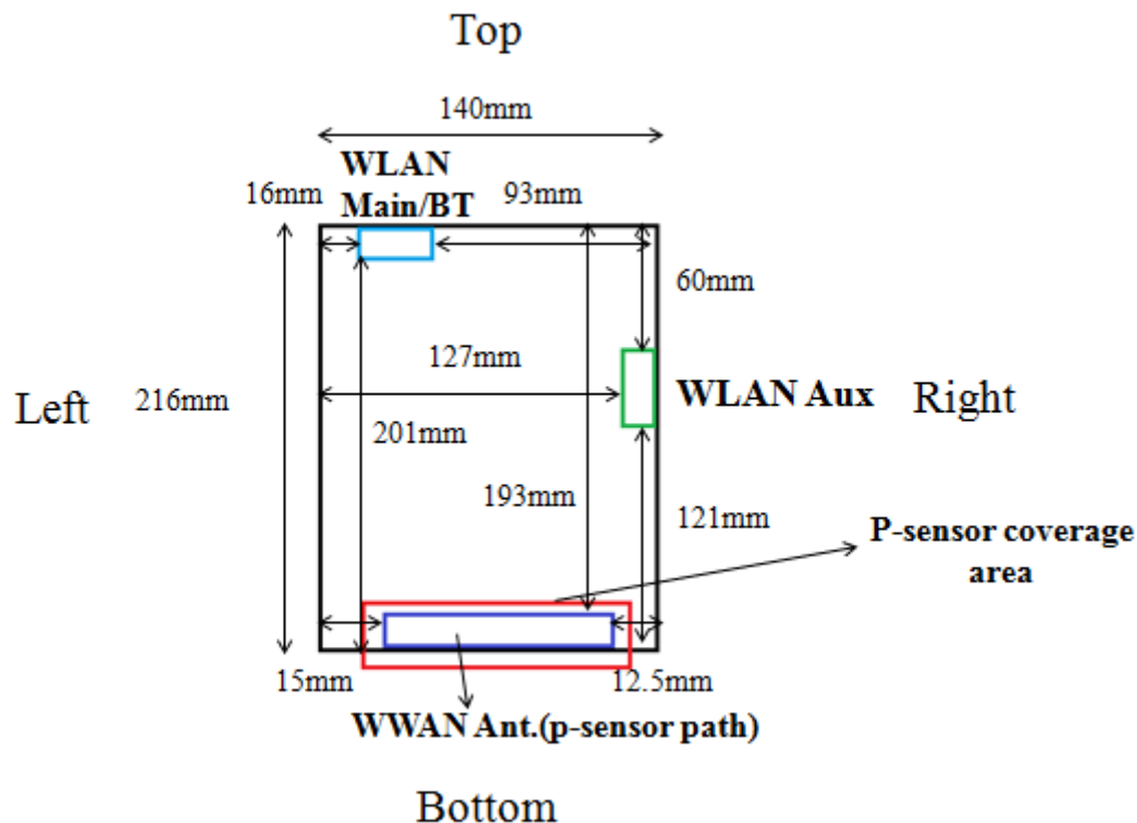
Fig.12 Antenna position of EUT (Front view)
