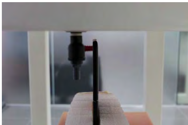
Fig.8 EUT Top side to flat phantom
