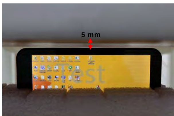
Fig.9 EUT Left side to flat phantom
