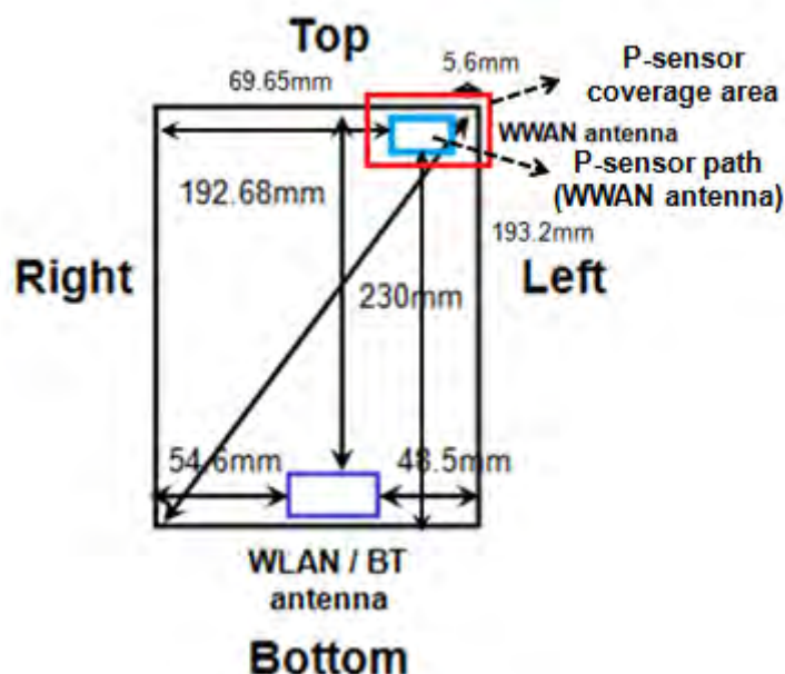
Fig.12 Antenna position of EUT (Back view)
