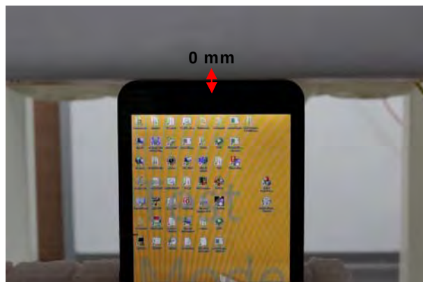
Fig.5 EUT Bottom side to flat phantom
