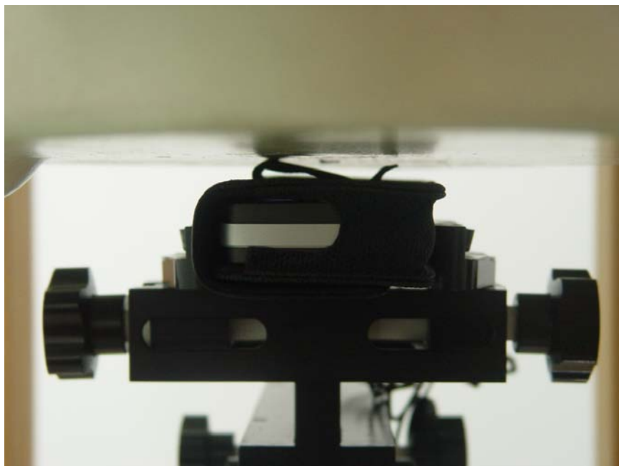
Fig. 9.9 Keypad Up with Holster Touch
