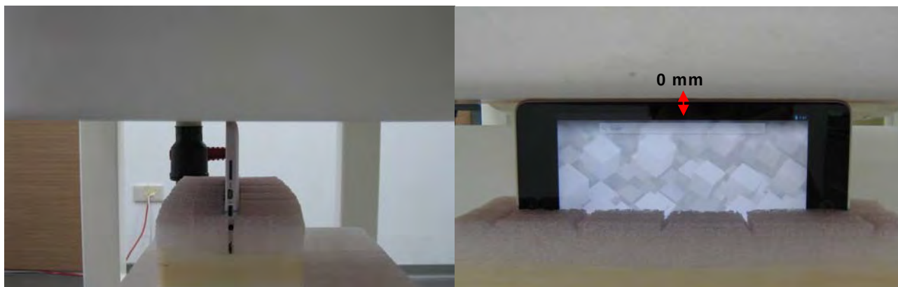
Fig.4 EUT Right side to flat phantom
