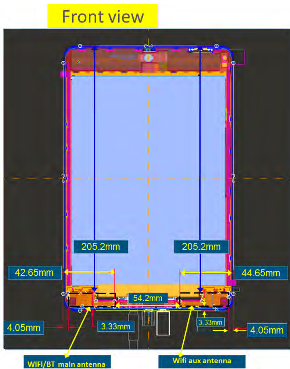
Fig.9 Antenna position of EUT
