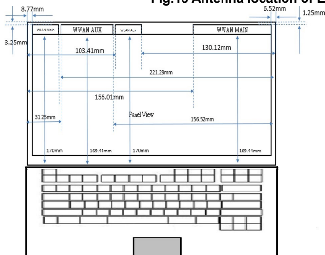
Fig.18 Antenna location of EUT (Tablet mode)
