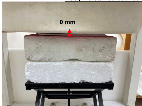
Fig.8 With_Keyboard_Back side
