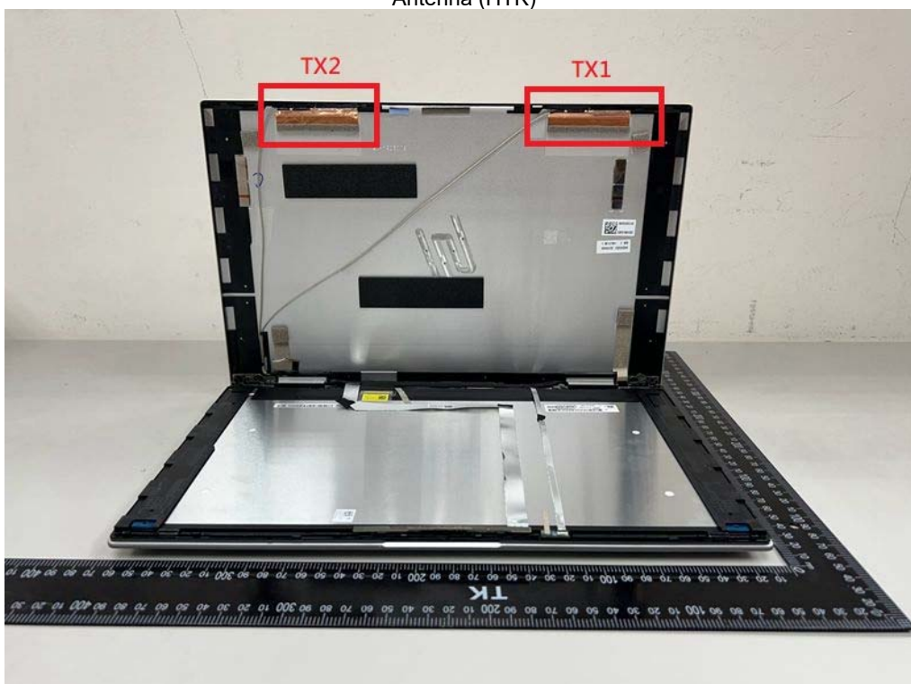
Antenna (HTK)
