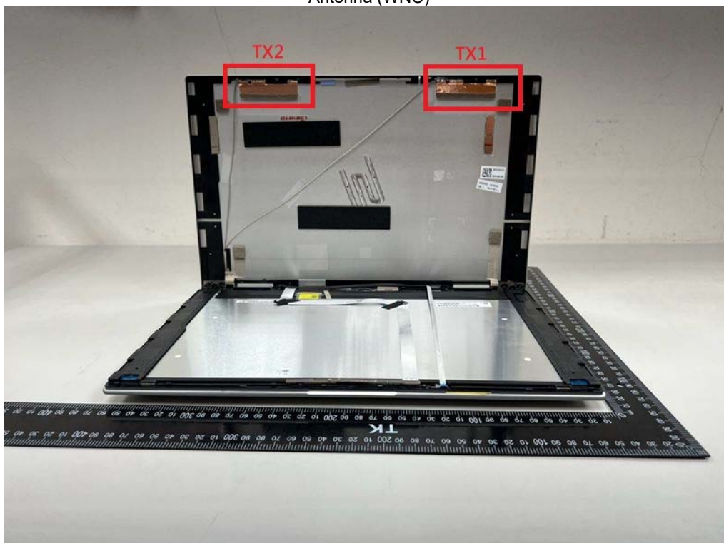
Antenna (WNC)
