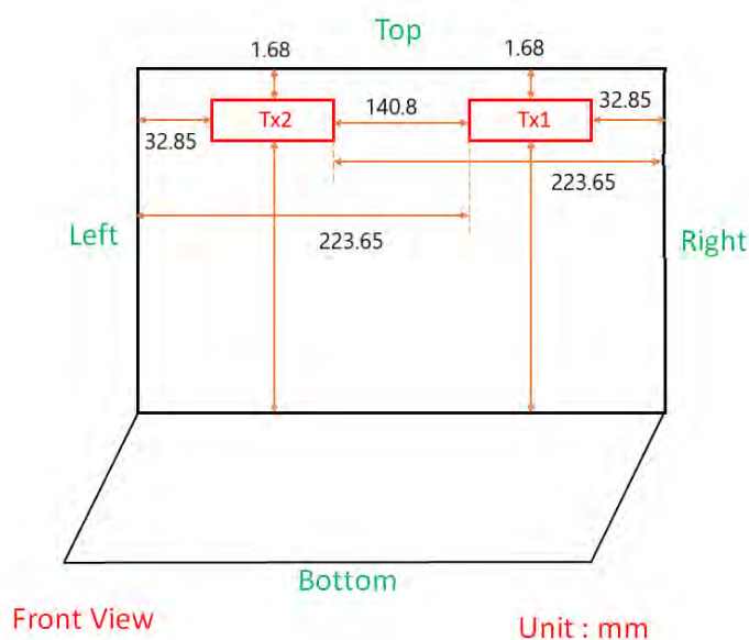
Fig.11 Antenna position of EUT (Laptop mode)
