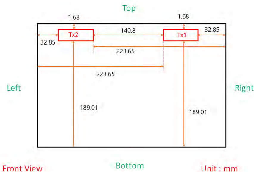
Fig.10 Antenna position of EUT (Tablet mode)
