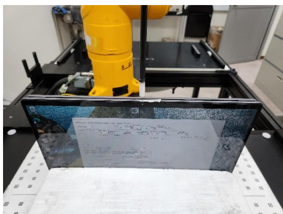
Photograph 3. PD, Top Edge, 2mm
