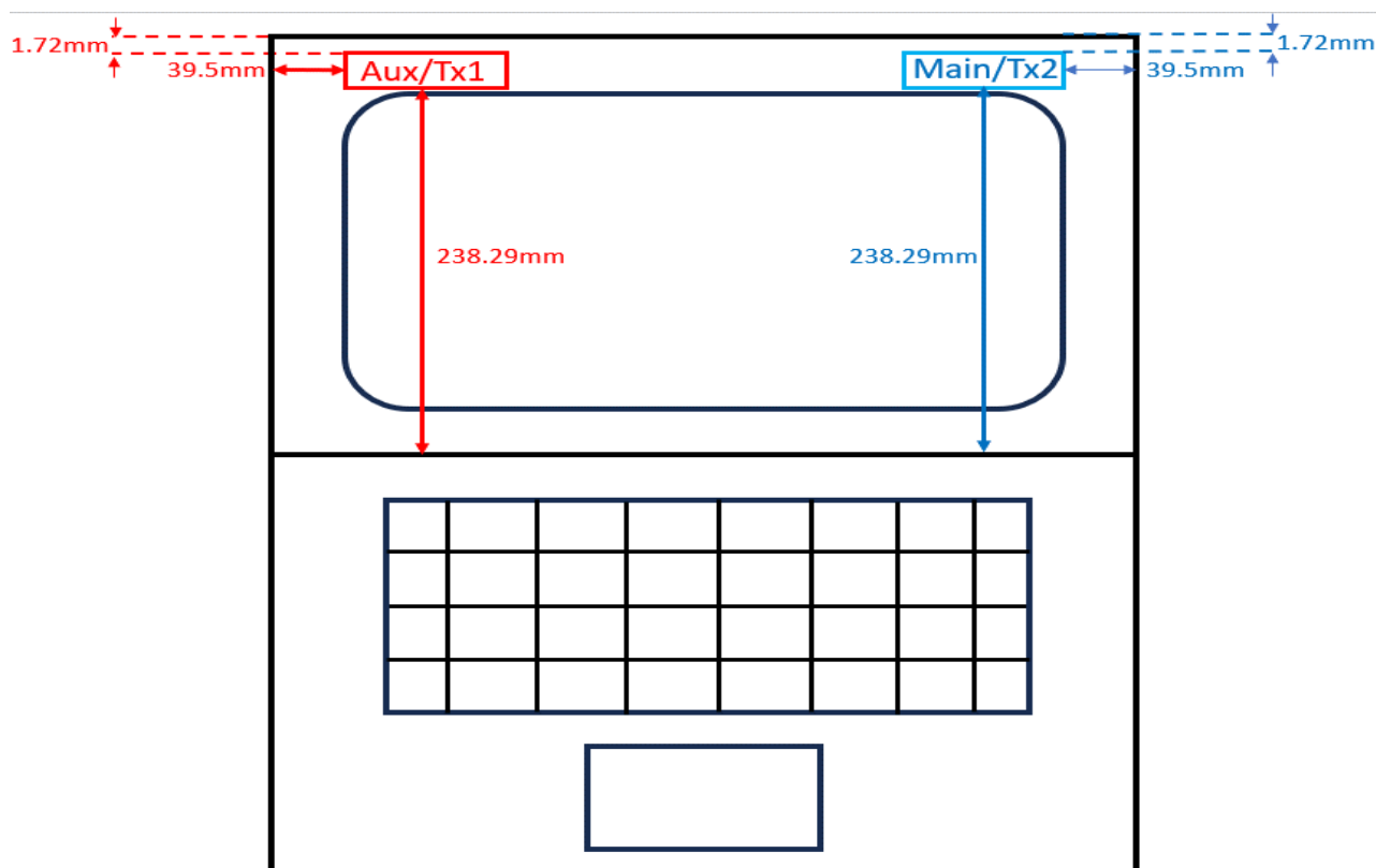
Photograph 13. Antenna position of EUT
