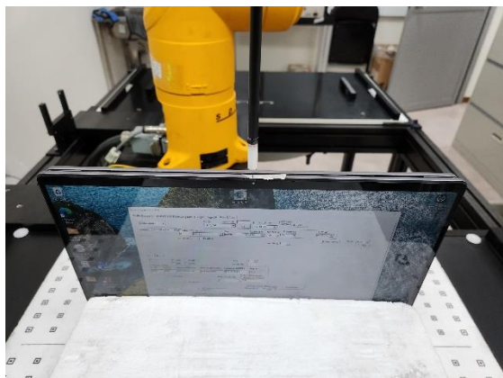
Photograph 9. PD, Top Edge, 2mm
