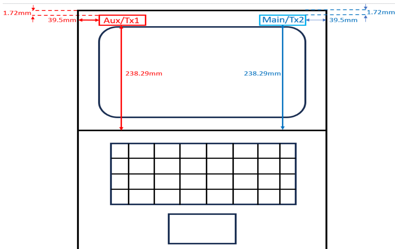
Photograph 13. Antenna position of EUT
