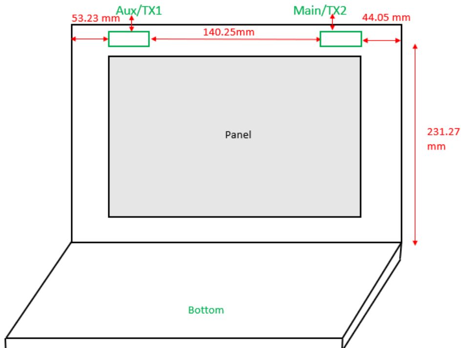
Photograph 13. Antenna position of EUT
