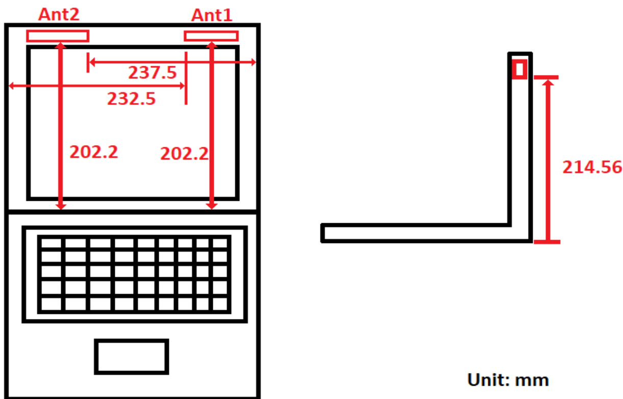
Photograph 11. Antenna position of EUT
