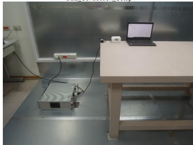
BLE_Conduction_Setup
