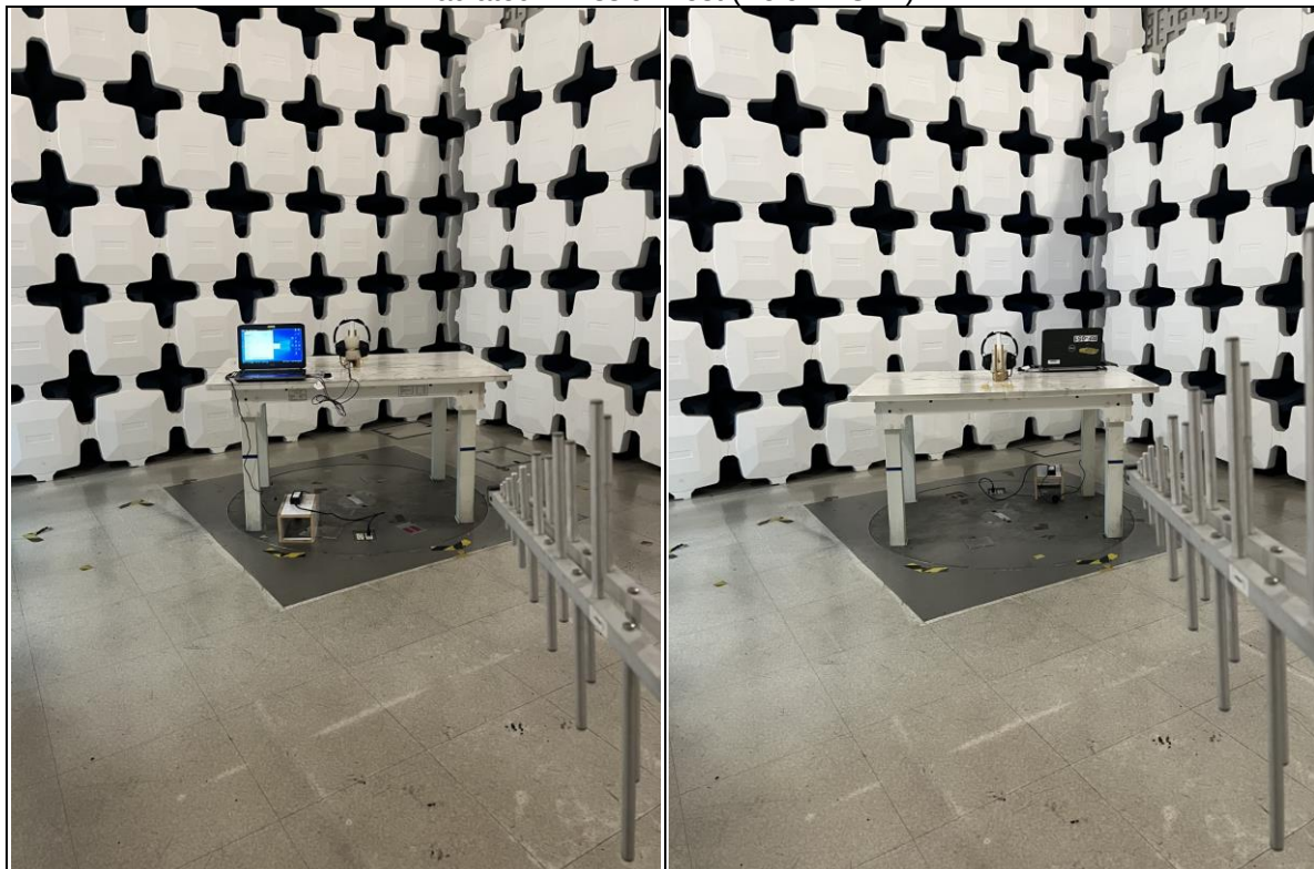
Radiated Emission Test (Below 1GHz)
