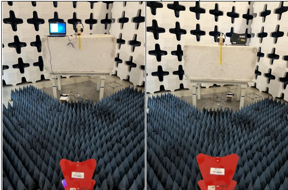
Radiated Emission Test (Above 1GHz)
