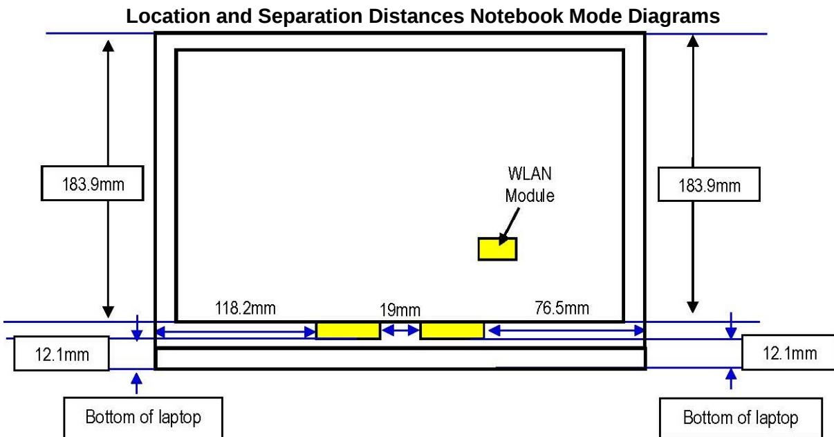
Location and Separation Distances Notebook Mode Diagrams
