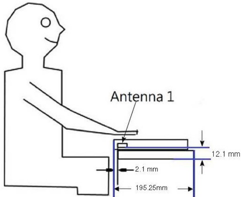
Location and Separation Distances Notebook Mode Diagrams
