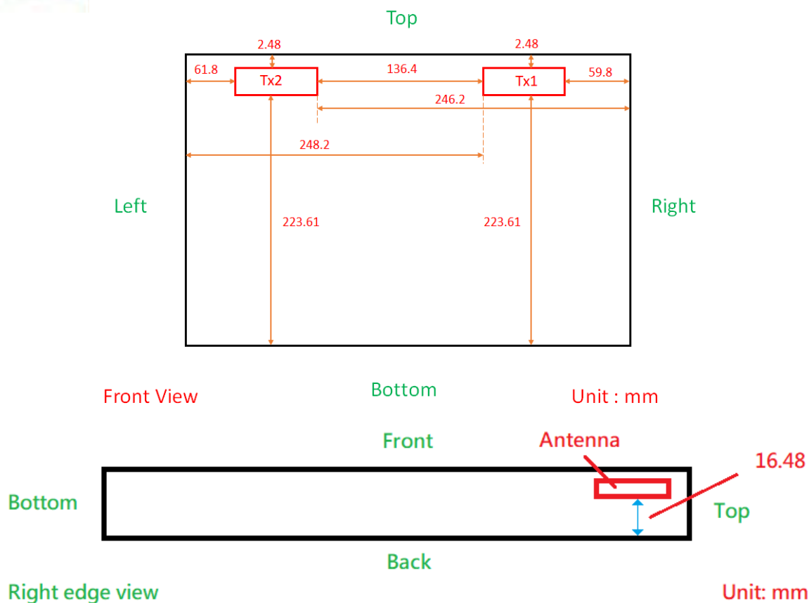
Fig.7 Antenna position of EUT (Tablet mode)
