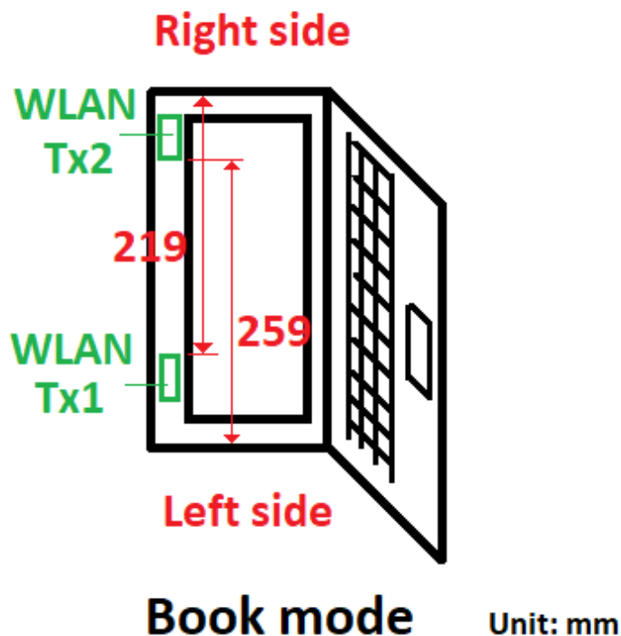
Fig.15 Antenna position of EUT (Book mode)
