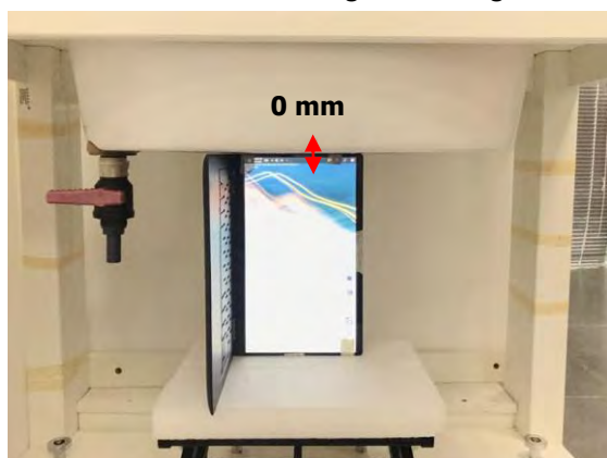
Fig.10 EUT Left side (Book mode) to flat phantom
