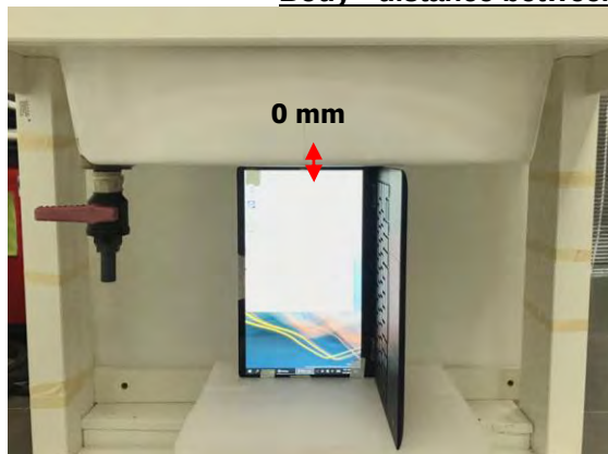
Fig.9 EUT Right side (Book mode) to flat phantom
