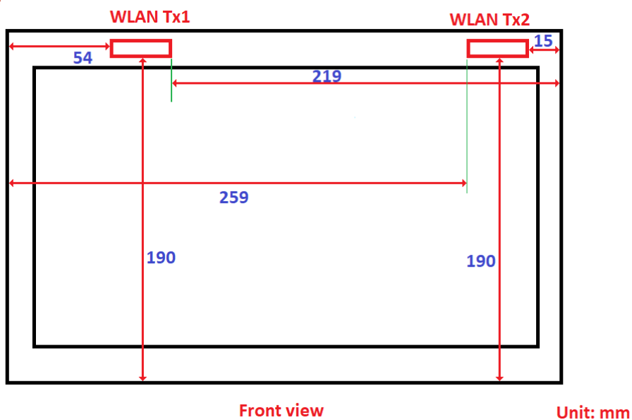
Fig.13 Antenna position of EUT (Tablet mode)
