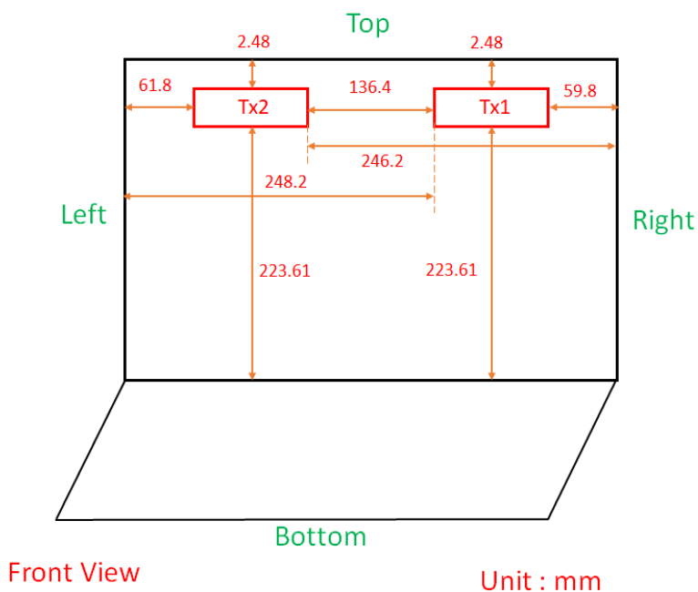
Fig.11 Antenna position of EUT (Laptop mode)
