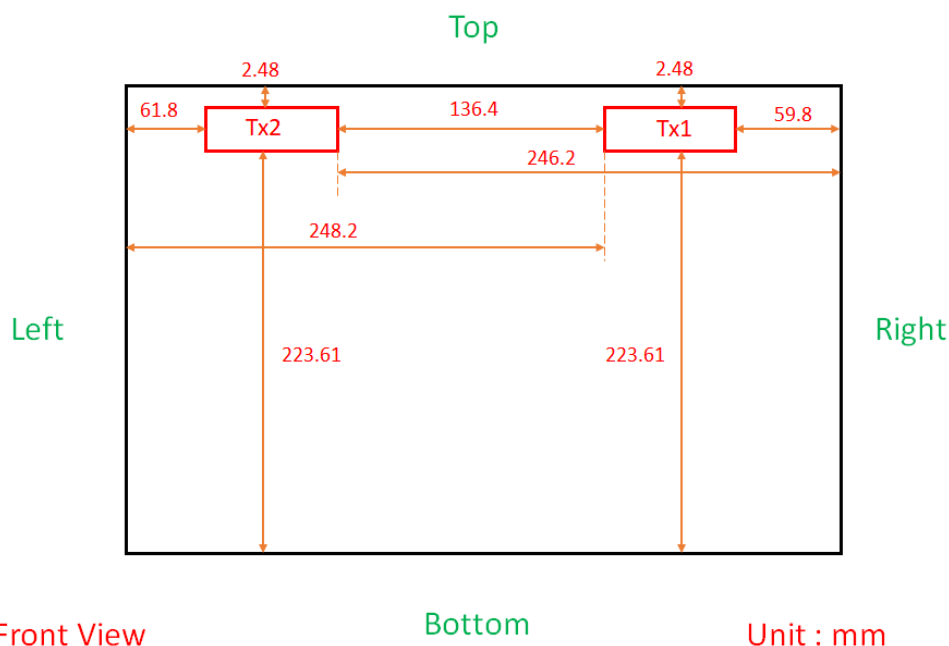
Fig.10 Antenna position of EUT (Tablet mode)
