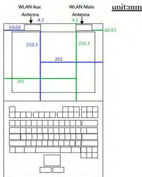
Fig.11 Antenna location of EUT (laptop mode)
