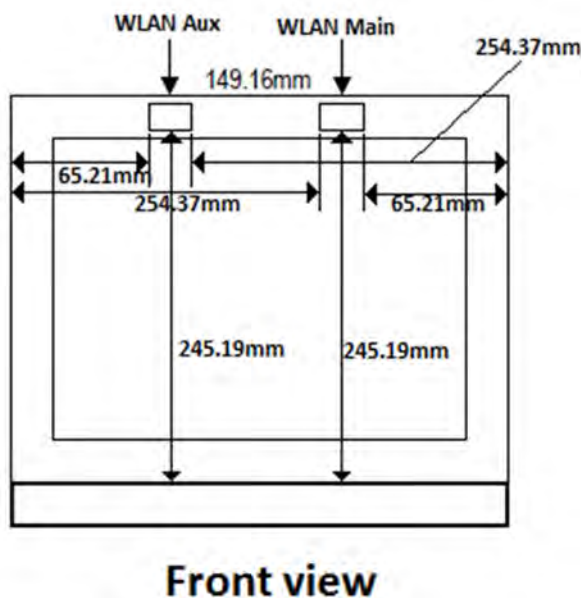
Fig.11 Antenna position of EUT ( front view )
