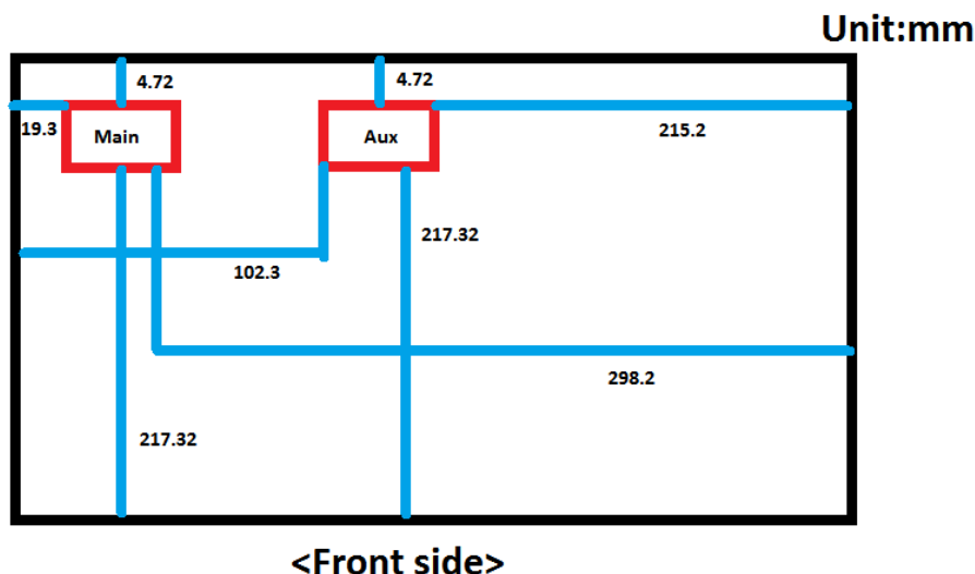
Fig.8 Antenna location of EUT (tablet mode)
