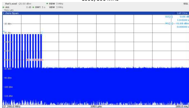
Figure 8.2-19: Deactivation time, OHF, 9 switch/3 position DIP switch, 1993-1995, 390 MHz
