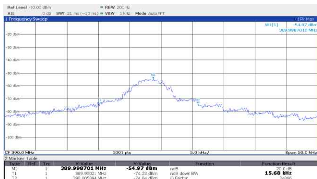
Figure 8.4-13: 20 dB bandwidth, Chamberlain, Yellow learn button, Security+2.0®, 2011-current, 390 MHz
