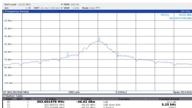
Figure 8.4-1: 20 dB bandwidth, Guardian, fixed learn code, 303 MHz
