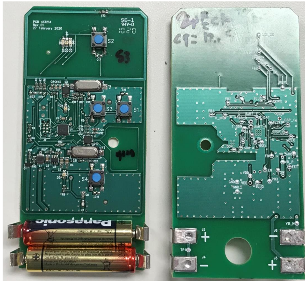
PCB Front
