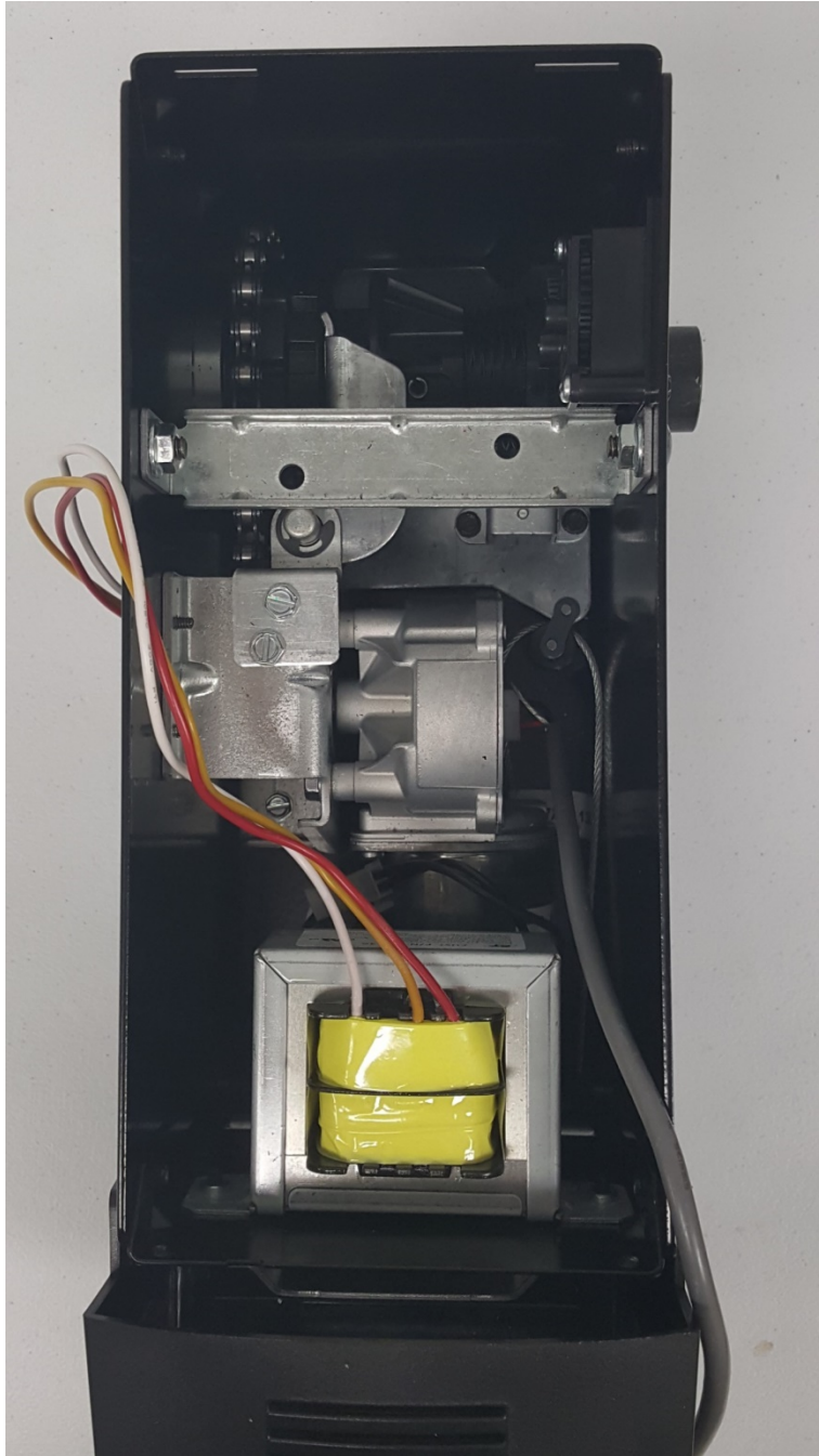
INTERNAL VIEW – WITHOUT FRONT PANEL
