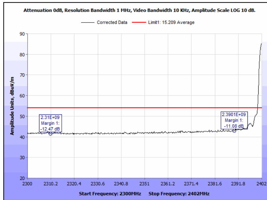
Plot 23. Radiated Restricted Band Edge, Average
