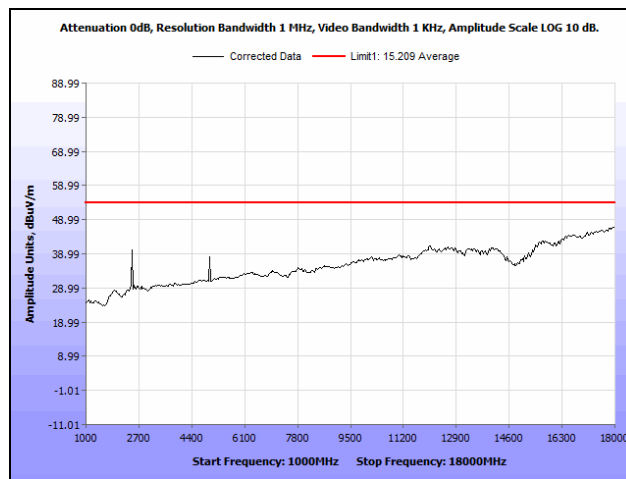
Plot 15. Radiated Spurious Emissions, High Channel, 1 GHz – 18 GHz, Average
