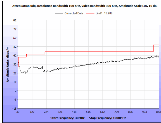
Plot 8. Radiated Spurious Emissions, Low Channel, 30 MHz – 1 GHz
