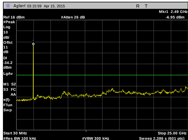
Plot 22. Conducted Spurious Emissions, High Channel, 30 MHz – 25 GHz
