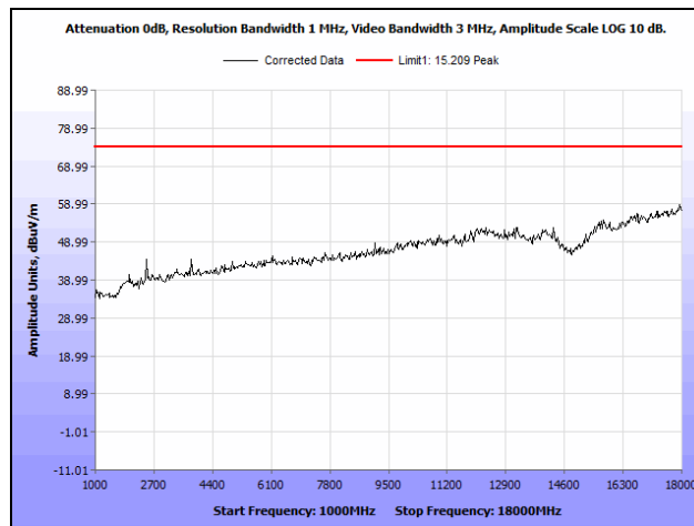
Plot 16. Radiated Spurious Emissions, High Channel, 1 GHz – 18 GHz, Peak
