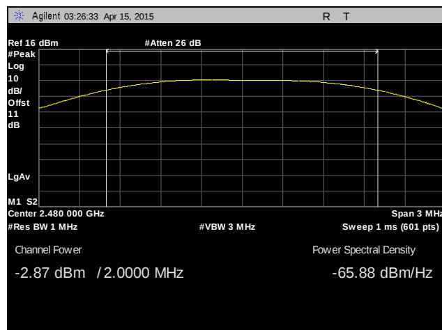
Plot 7. Peak Power Output, High Channel
