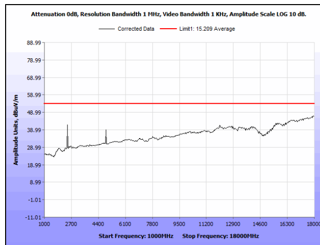
Plot 12. Radiated Spurious Emissions, Mid Channel, 1 GHz – 18 GHz, Average
