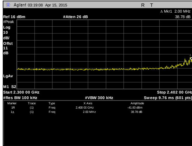
Plot 23. Conducted Band Edge, Low, Channel
