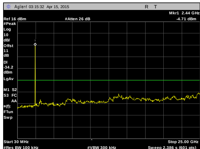
Plot 21. Conducted Spurious Emissions, Mid Channel, 30 MHz – 25 GHz
