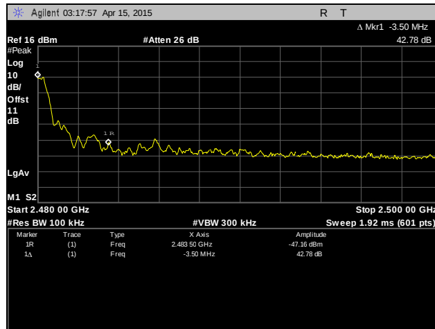
Plot 24. Conducted Band Edge, High Channel
