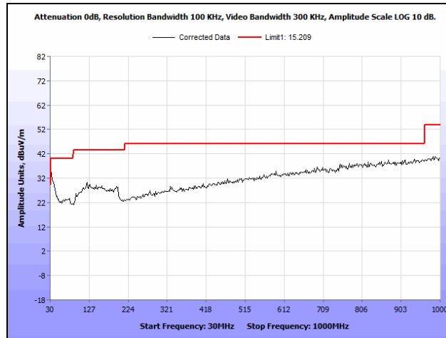
Plot 14. Radiated Spurious Emissions, High Channel, 30 MHz – 1 GHz
