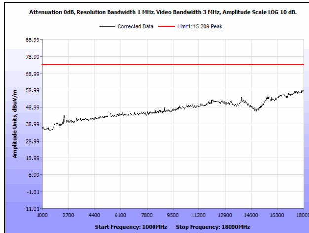
Plot 10. Radiated Spurious Emissions, Low Channel, 1 GHz – 18 GHz, Peak
