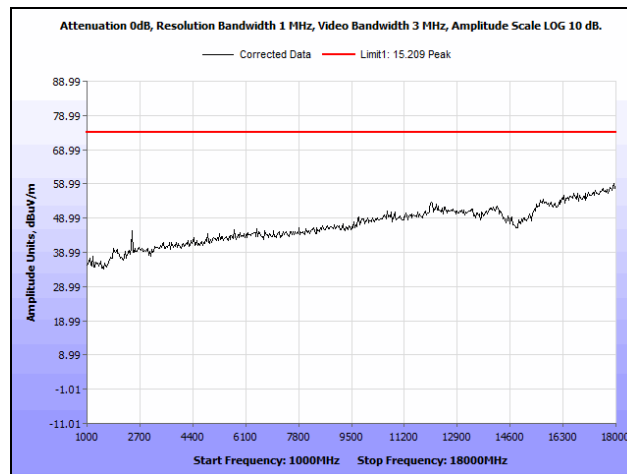
Plot 13. Radiated Spurious Emissions, Mid Channel, 1 GHz – 18 GHz, Peak
