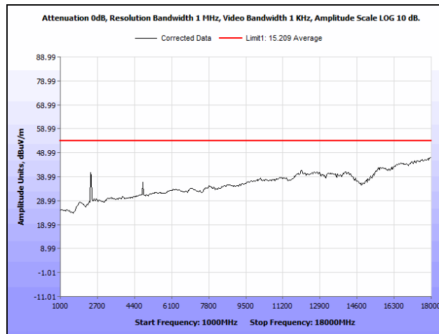
Plot 9. Radiated Spurious Emissions, Low Channel, 1 GHz – 18 GHz, Average
