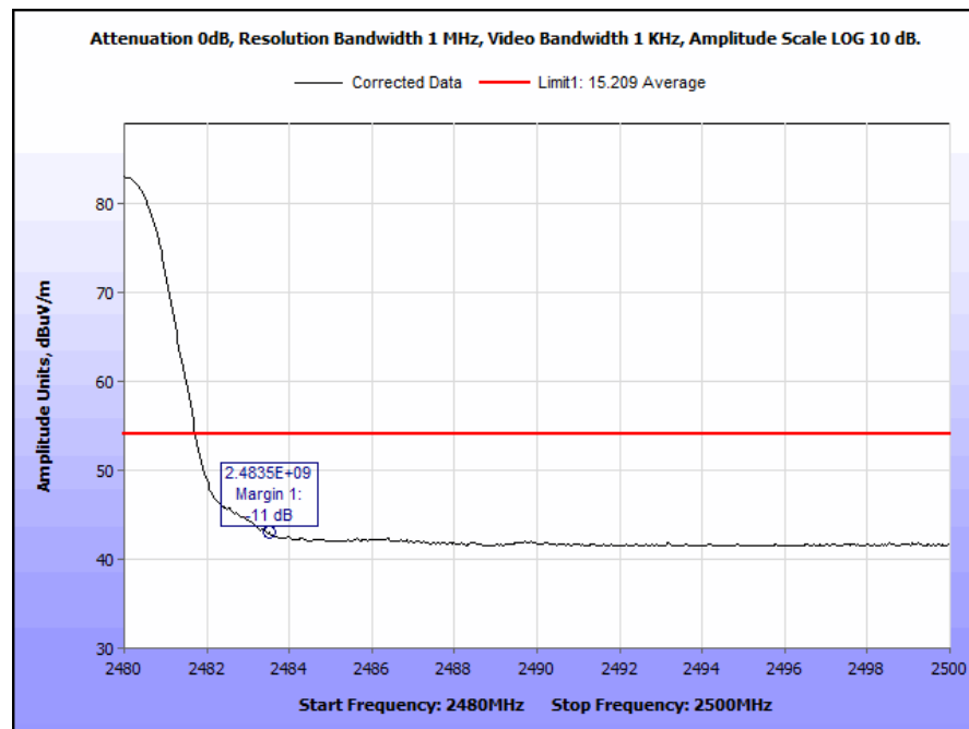
Plot 17. Radiated Restricted Band Edge, High Channel, Average
