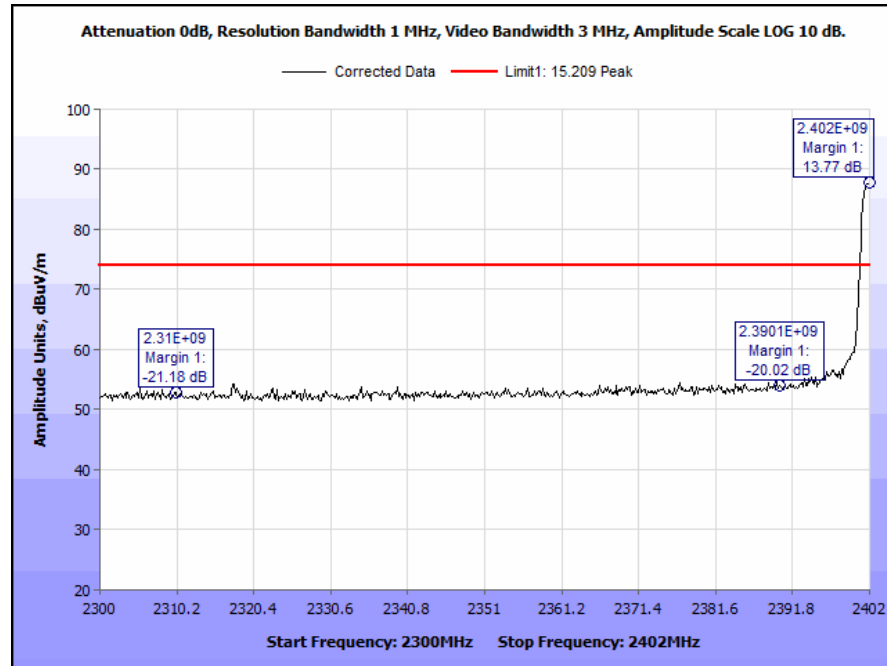
Plot 19. Radiated Restricted Band Edge, Peak
