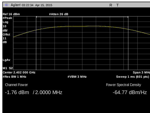
Plot 5. Peak Power Output, Low Channel
