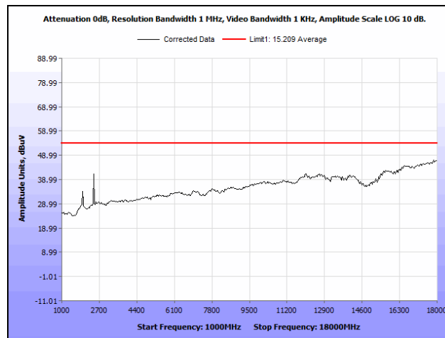
Plot 16. Radiated Spurious Emissions, Mid Channel, 1 GHz – 18 GHz, Average
