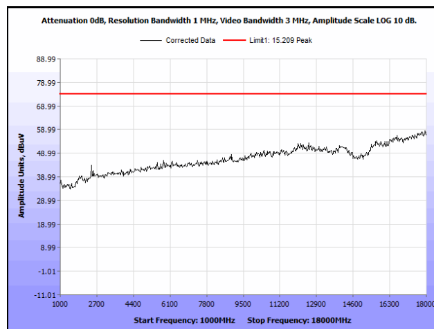
Plot 17. Radiated Spurious Emissions, Mid Channel, 1 GHz – 18 GHz, Peak
