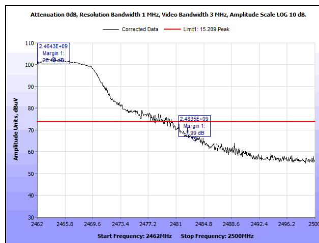
Plot 60. Radiated Restricted Band Edge, High Channel, Peak, 802.11g
