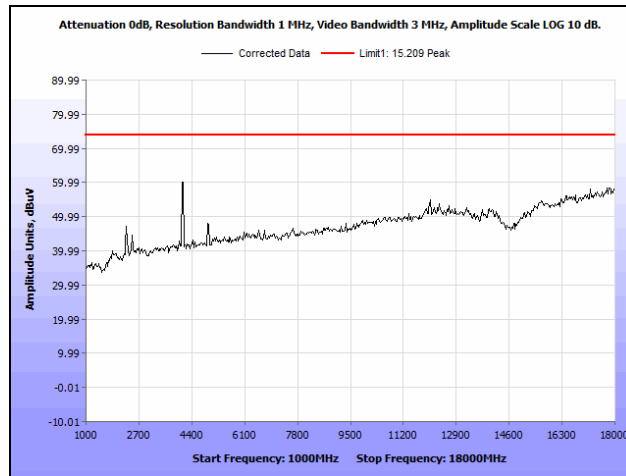
Plot 34. Radiated Spurious Emissions, High Channel, 802.11b, 1 GHz – 18 GHz, Peak
