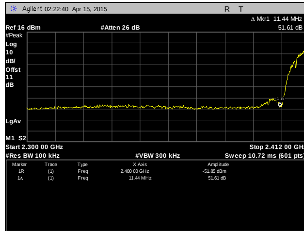
Plot 74. Conducted Band Edge, Low, Channel, 802.11b
