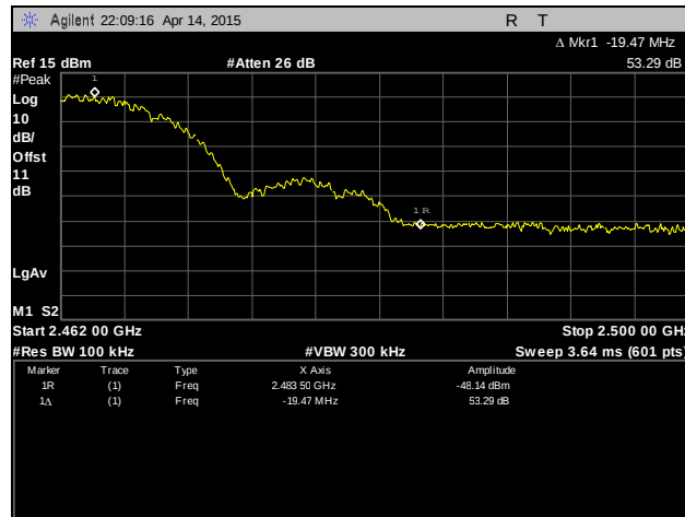
Plot 75. Conducted Band Edge, High Channel, 802.11b
