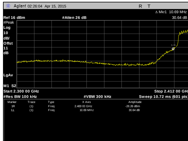
Plot 76. Conducted Band Edge, Low, Channel, 802.11g
