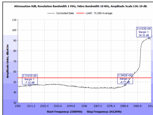
Plot 57. Radiated Restricted Band Edge, Low Channel, Average, 802.11g
