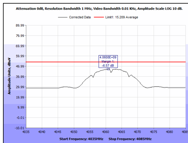
Plot 29. Radiated Spurious Emissions, Mid Channel, 802.11b, 1 GHz – 18 GHz, Average, 4.06 GHz, Zoomed
