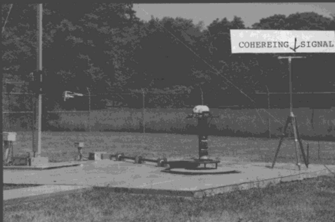
Radiated Emissions Testing
