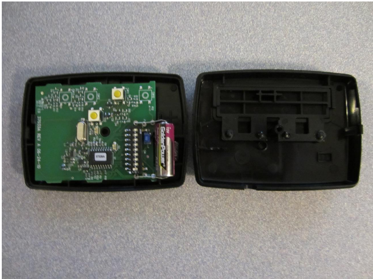
Figure 1: Internal View / PCB Top
