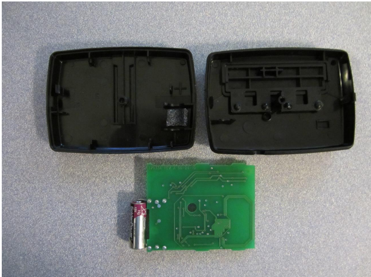
Figure 2: Internal View / PCB Bottom
