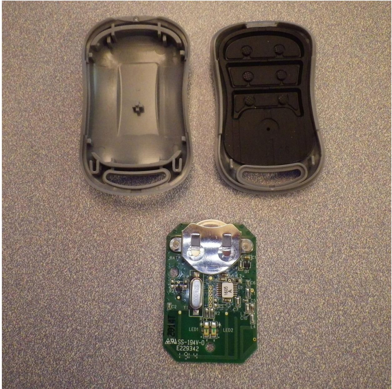
Figure 1: G3T-A Internal / PCB Top
