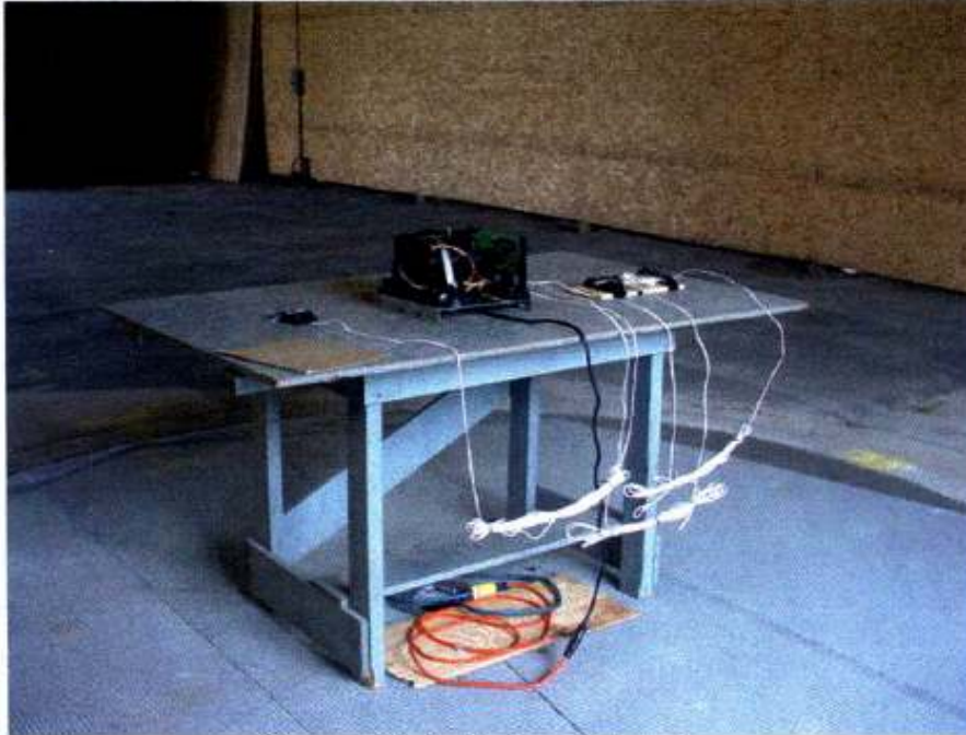
Photograph 1: Radiated Emissions
