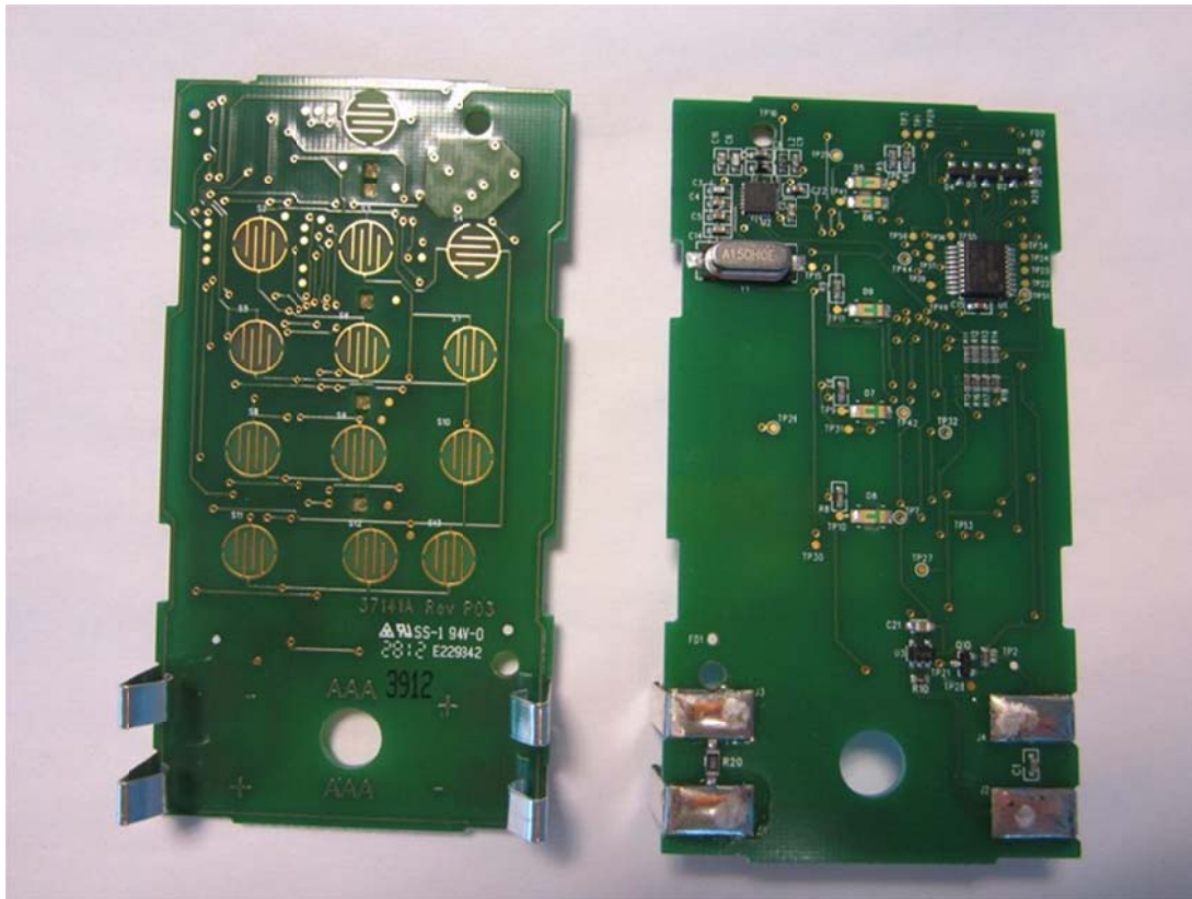
Front and back views of the circuit board.
